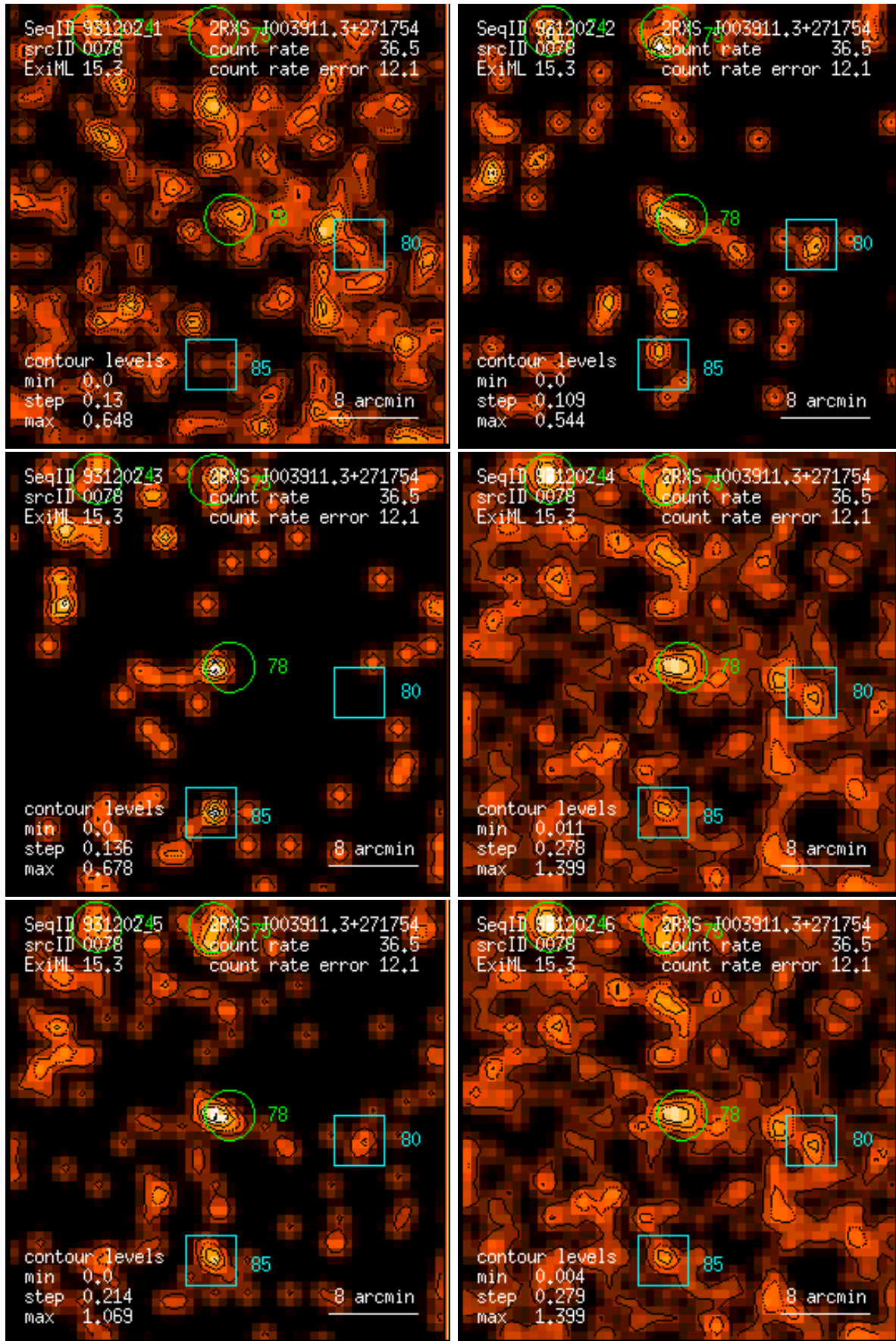
Figure 78: RASS 931202: detection 0078: band rate images, Gaussian filter: (1) PSPC channels 11 – 41, (2) 52 – 90, (3) 91 – 201, (4) 11 – 235, (5) 52 – 201, (6) 11 – 201. Broad band rates in counts/ks. Band rate contour levels in counts/ks/arcmin 2 .
