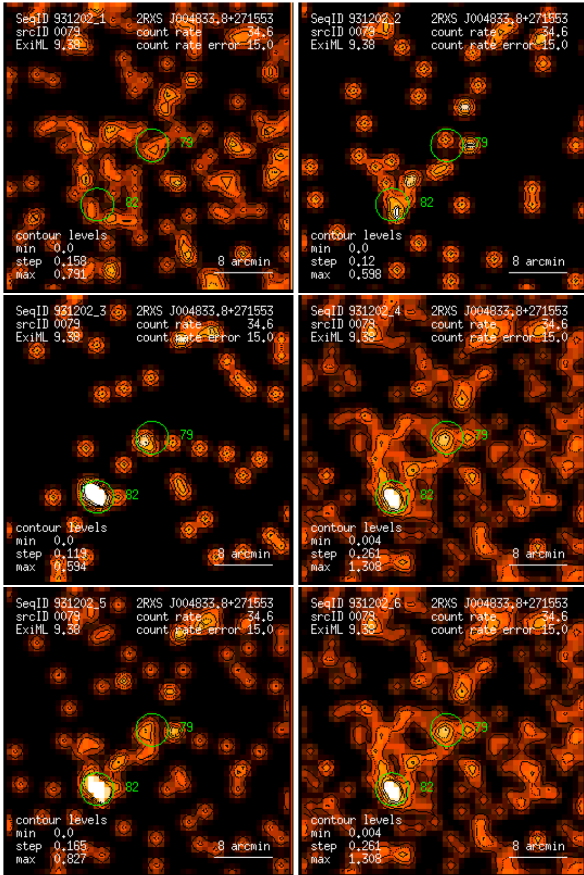
Figure 79: RASS 931202: detection 0079: band rate images, Gaussian filter: (1) PSPC channels 11 – 41, (2) 52 – 90, (3) 91 – 201, (4) 11 – 235, (5) 52 – 201, (6) 11 – 201. Broad band rates in counts/ks. Band rate contour levels in counts/ks/arcmin 2 .
