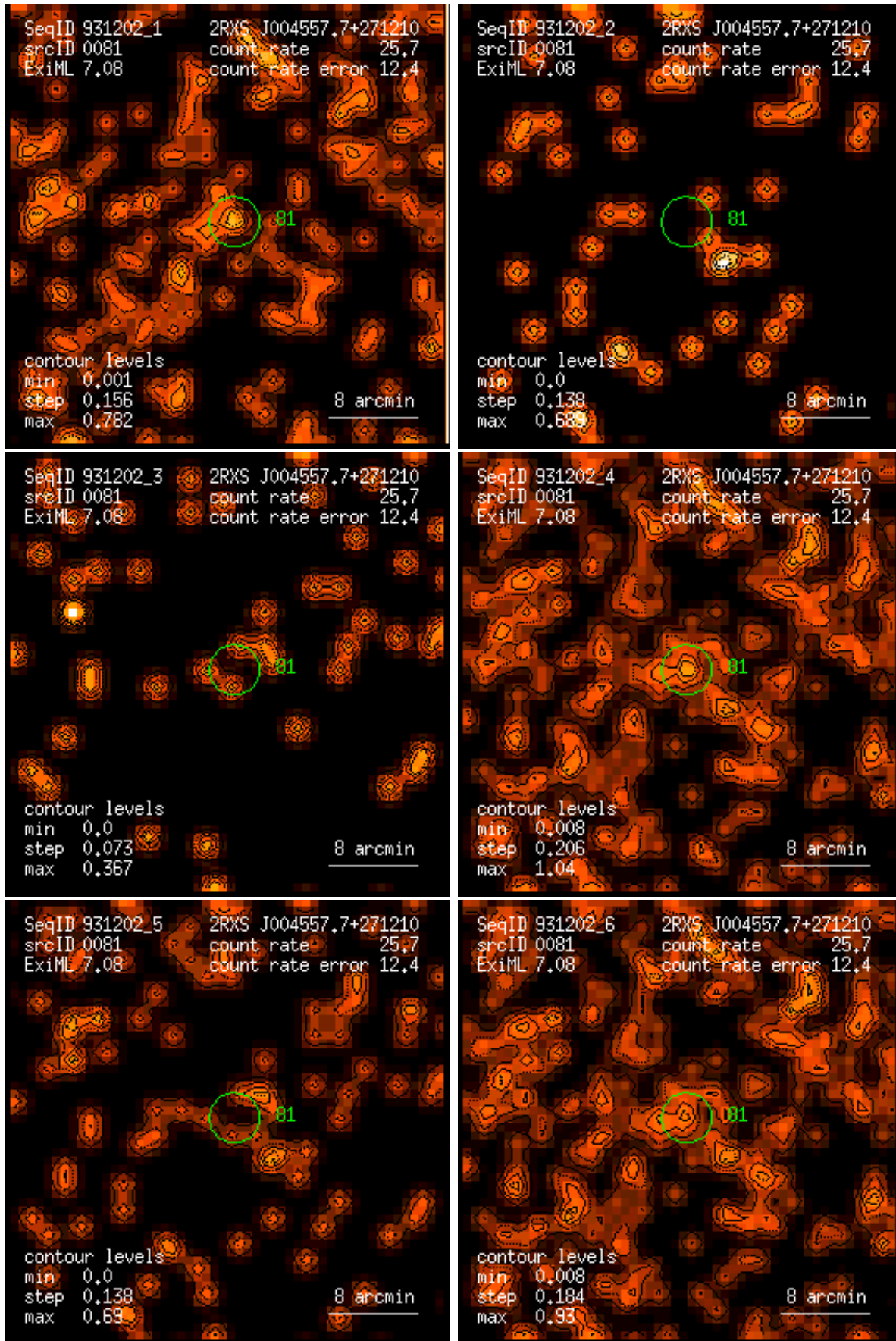
Figure 81: RASS 931202: detection 0081: band rate images, Gaussian filter: (1) PSPC channels 11 – 41, (2) 52 – 90, (3) 91 – 201, (4) 11 – 235, (5) 52 – 201, (6) 11 – 201. Broad band rates in counts/ks. Band rate contour levels in counts/ks/arcmin 2 .
