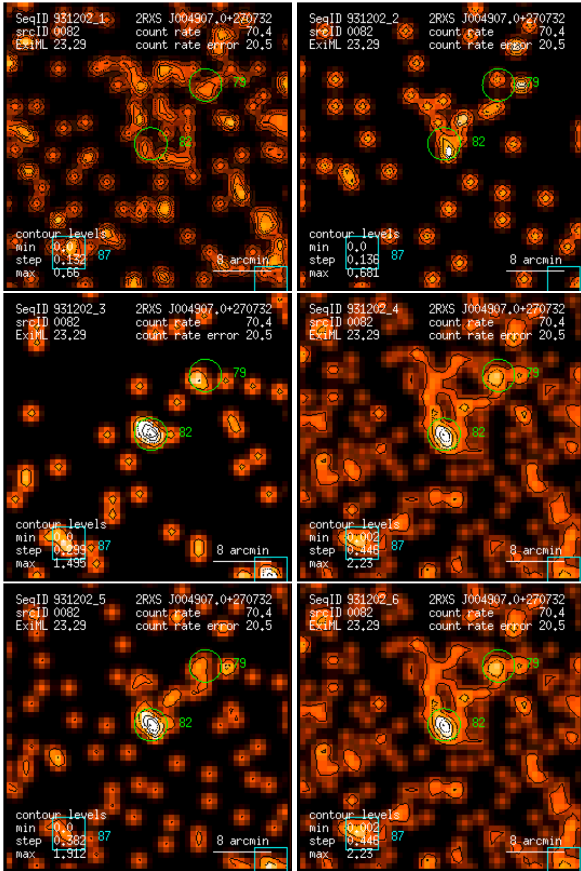
Figure 82: RASS 931202: detection 0082: band rate images, Gaussian filter: (1) PSPC channels 11 – 41, (2) 52 – 90, (3) 91 – 201, (4) 11 – 235, (5) 52 – 201, (6) 11 – 201. Broad band rates in counts/ks. Band rate contour levels in counts/ks/arcmin 2 .
