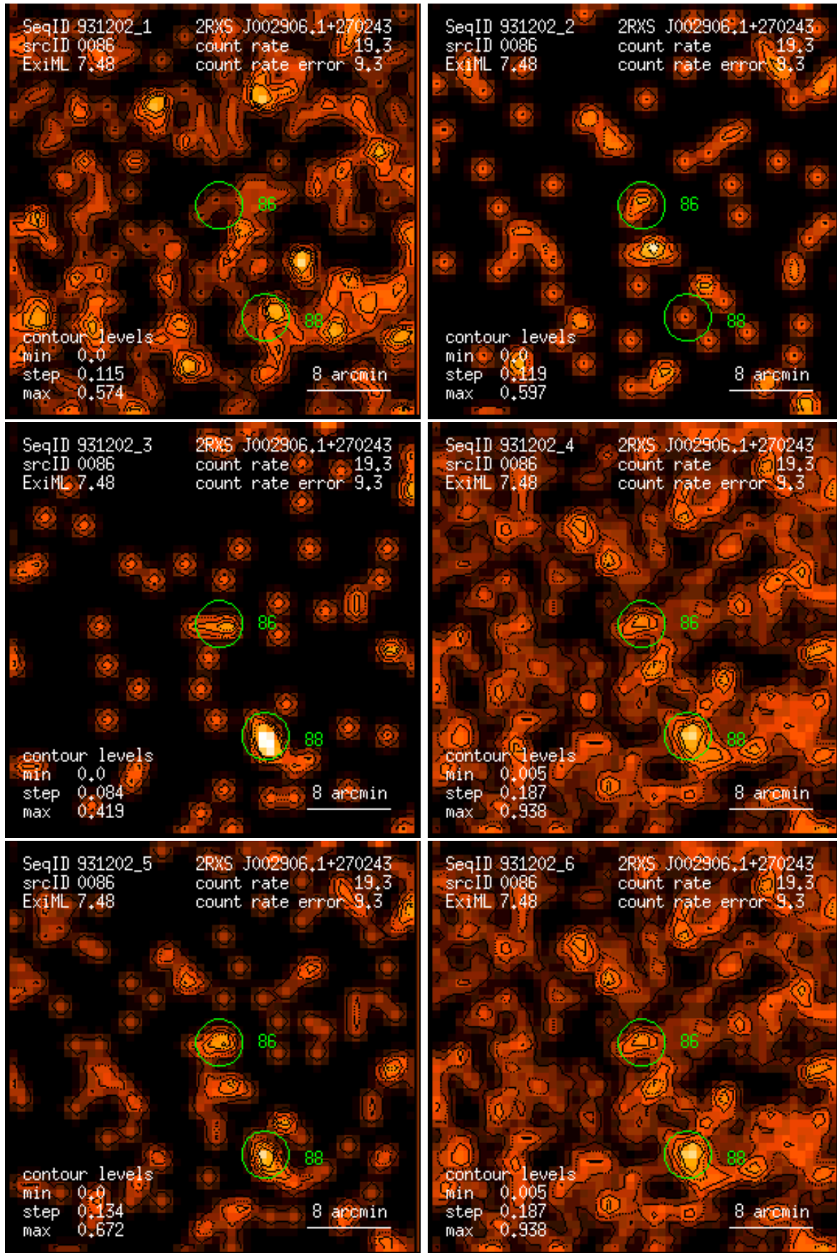
Figure 86: RASS 931202: detection 0086: band rate images, Gaussian filter: (1) PSPC channels 11 – 41, (2) 52 – 90, (3) 91 – 201, (4) 11 – 235, (5) 52 – 201, (6) 11 – 201. Broad band rates in counts/ks. Band rate contour levels in counts/ks/arcmin 2 .
