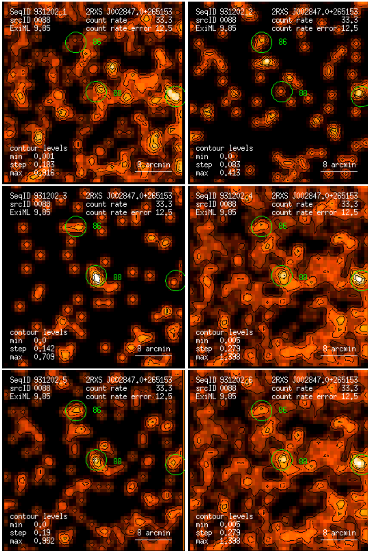
Figure 88: RASS 931202: detection 0088: band rate images, Gaussian filter: (1) PSPC channels 11 – 41, (2) 52 – 90, (3) 91 – 201, (4) 11 – 235, (5) 52 – 201, (6) 11 – 201. Broad band rates in counts/ks. Band rate contour levels in counts/ks/arcmin 2 .
