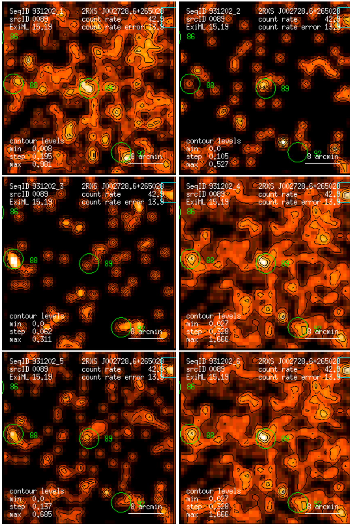
Figure 89: RASS 931202: detection 0089: band rate images, Gaussian filter: (1) PSPC channels 11 – 41, (2) 52 – 90, (3) 91 – 201, (4) 11 – 235, (5) 52 – 201, (6) 11 – 201. Broad band rates in counts/ks. Band rate contour levels in counts/ks/arcmin 2 .
