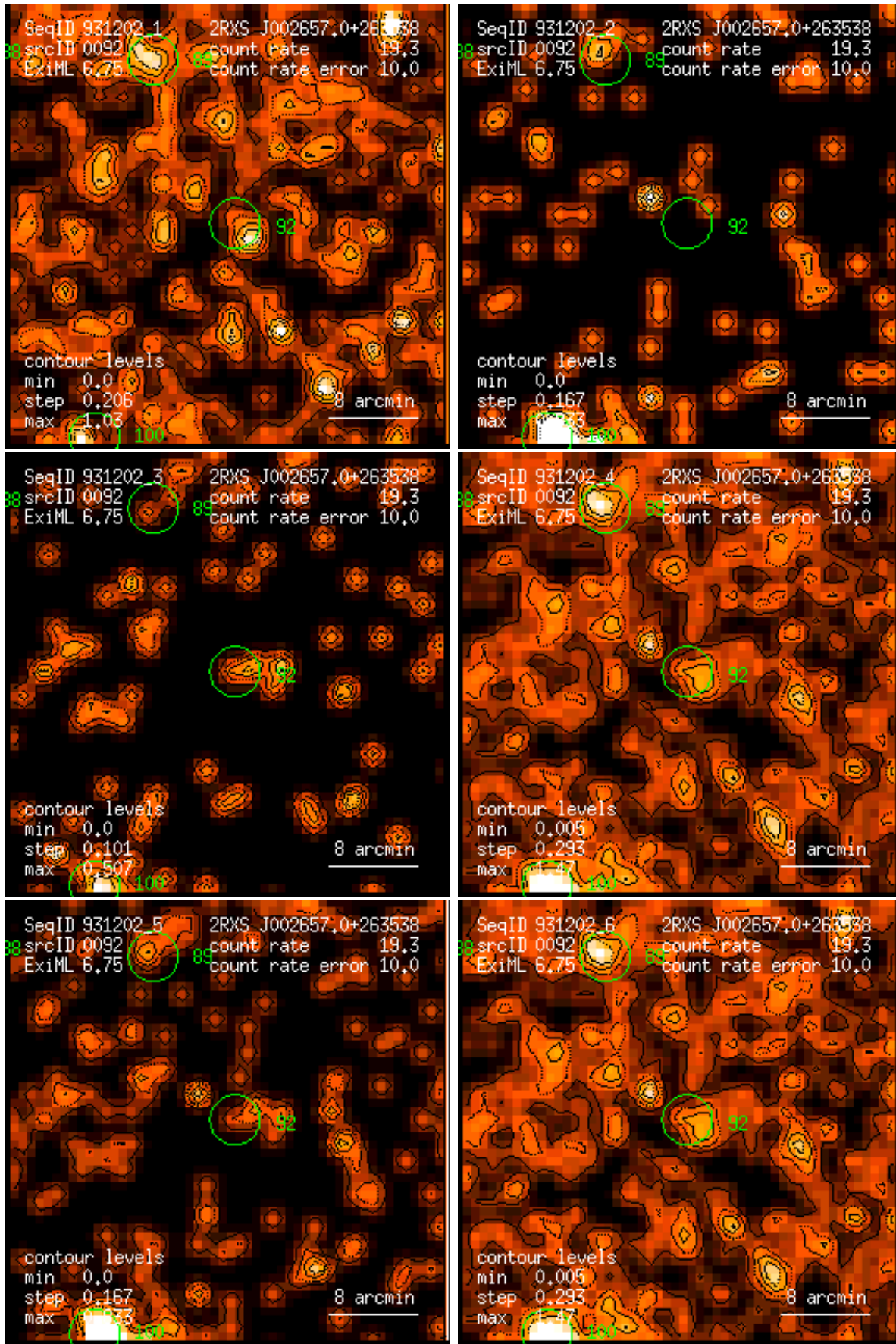
Figure 92: RASS 931202: detection 0092: band rate images, Gaussian filter: (1) PSPC channels 11 – 41, (2) 52 – 90, (3) 91 – 201, (4) 11 – 235, (5) 52 – 201, (6) 11 – 201. Broad band rates in counts/ks. Band rate contour levels in counts/ks/arcmin 2 .
