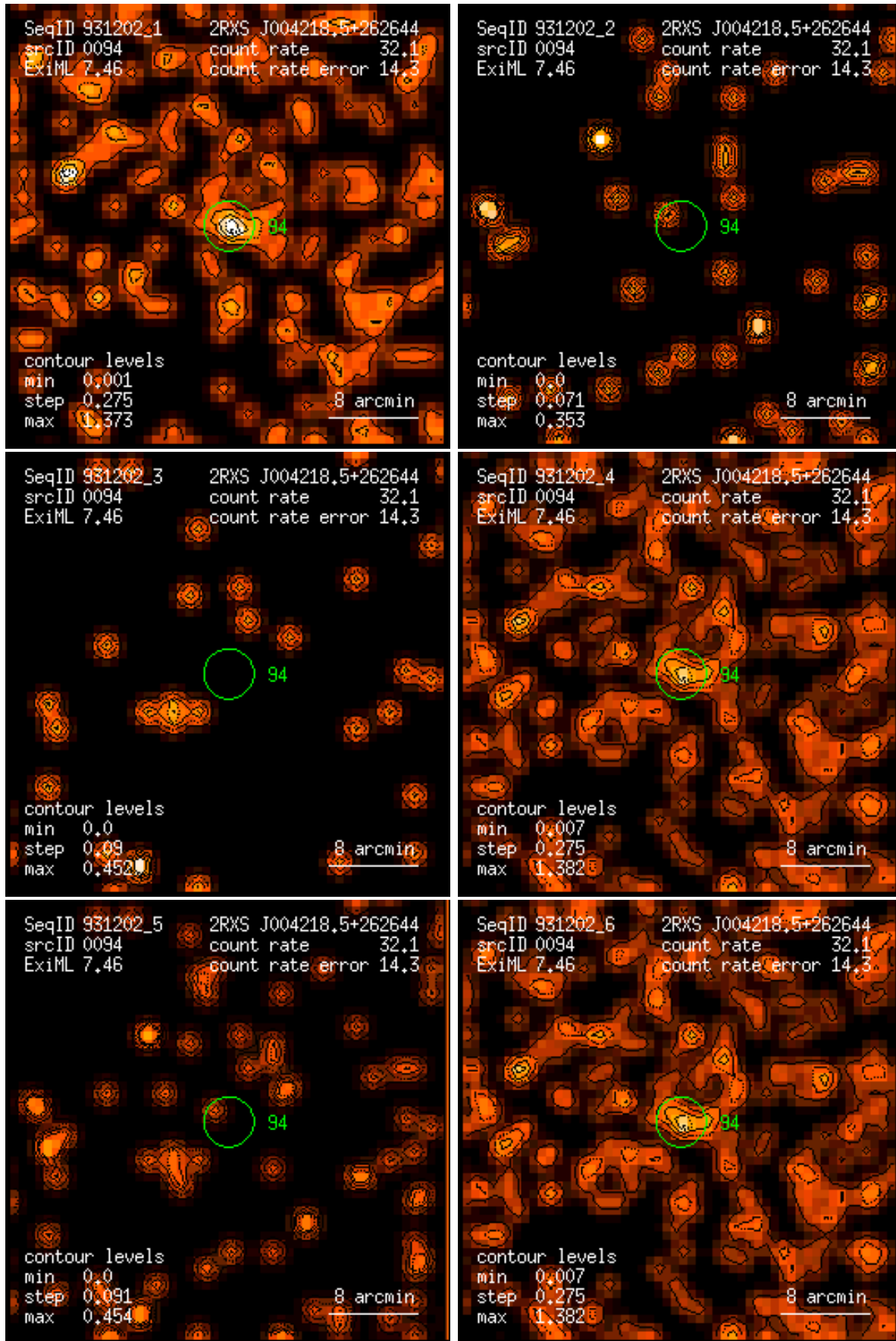
Figure 94: RASS 931202: detection 0094: band rate images, Gaussian filter: (1) PSPC channels 11 – 41, (2) 52 – 90, (3) 91 – 201, (4) 11 – 235, (5) 52 – 201, (6) 11 – 201. Broad band rates in counts/ks. Band rate contour levels in counts/ks/arcmin 2 .
