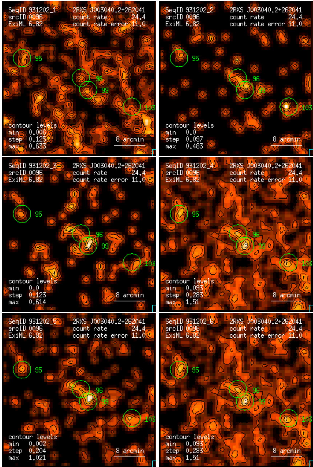
Figure 96: RASS 931202: detection 0096: band rate images, Gaussian filter: (1) PSPC channels 11 – 41, (2) 52 – 90, (3) 91 – 201, (4) 11 – 235, (5) 52 – 201, (6) 11 – 201. Broad band rates in counts/ks. Band rate contour levels in counts/ks/arcmin 2 .
