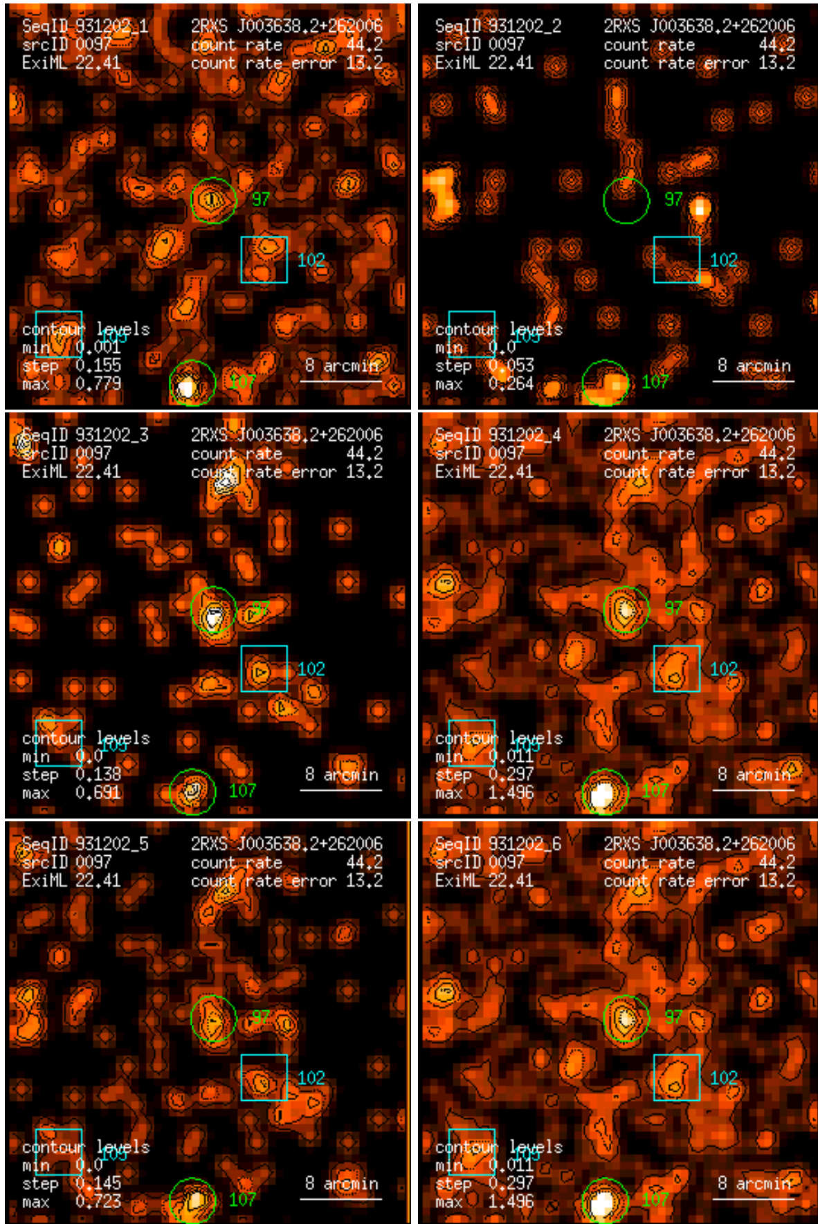
Figure 97: RASS 931202: detection 0097: band rate images, Gaussian filter: (1) PSPC channels 11 – 41, (2) 52 – 90, (3) 91 – 201, (4) 11 – 235, (5) 52 – 201, (6) 11 – 201. Broad band rates in counts/ks. Band rate contour levels in counts/ks/arcmin 2 .
