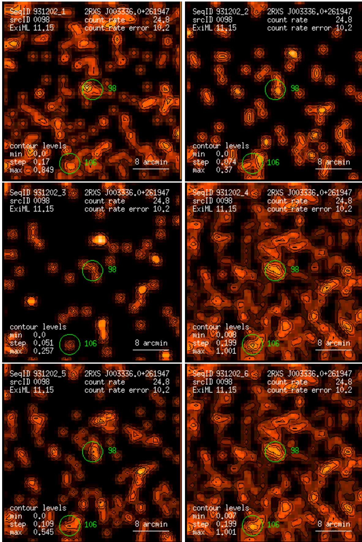
Figure 98: RASS 931202: detection 0098: band rate images, Gaussian filter: (1) PSPC channels 11 – 41, (2) 52 – 90, (3) 91 – 201, (4) 11 – 235, (5) 52 – 201, (6) 11 – 201. Broad band rates in counts/ks. Band rate contour levels in counts/ks/arcmin 2 .
