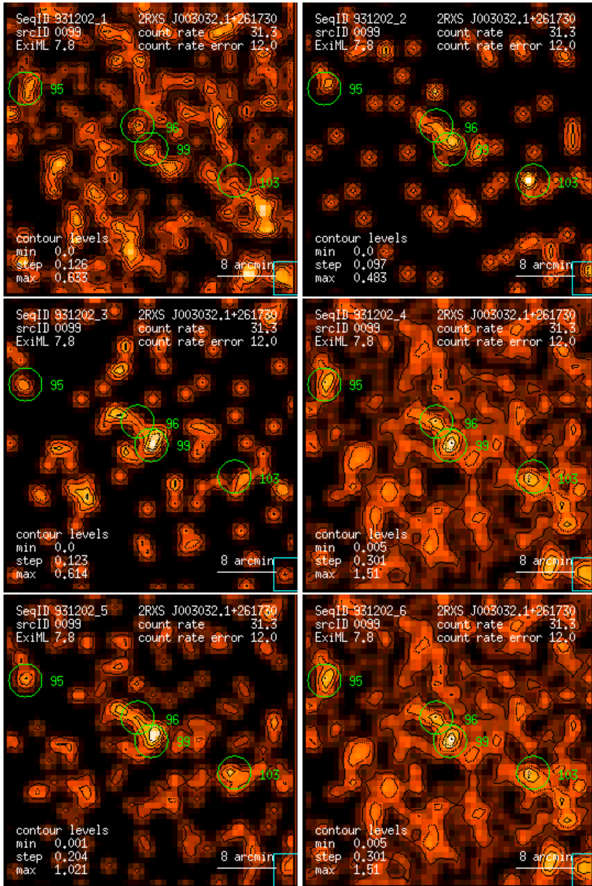
Figure 99: RASS 931202: detection 0099: band rate images, Gaussian filter: (1) PSPC channels 11 – 41, (2) 52 – 90, (3) 91 – 201, (4) 11 – 235, (5) 52 – 201, (6) 11 – 201. Broad band rates in counts/ks. Band rate contour levels in counts/ks/arcmin 2 .
