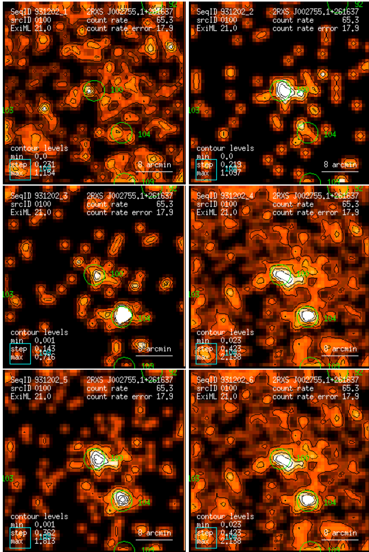
Figure 100: RASS 931202: detection 0100: band rate images, Gaussian filter: (1) PSPC channels 11 – 41, (2) 52 – 90, (3) 91 – 201, (4) 11 – 235, (5) 52 – 201, (6) 11 – 201. Broad band rates in counts/ks. Band rate contour levels in counts/ks/arcmin 2 .
