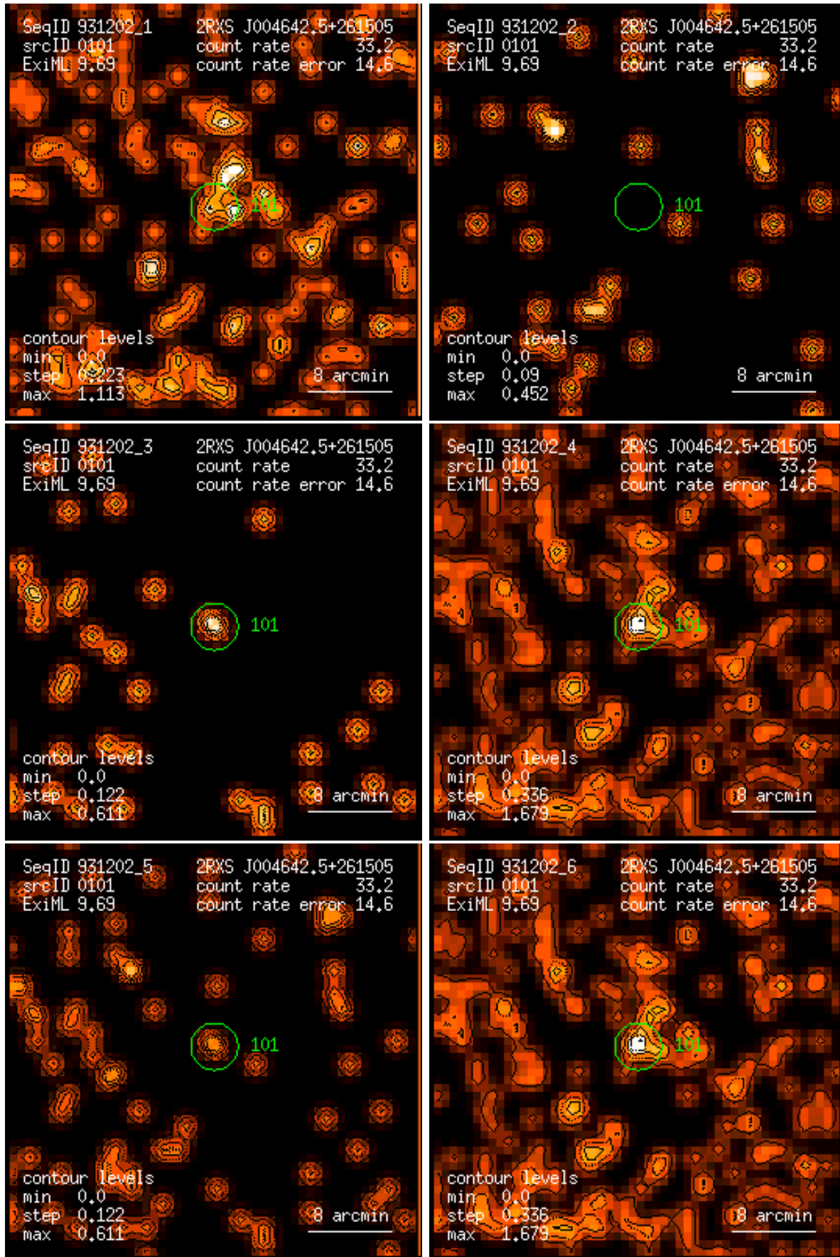
Figure 101: RASS 931202: detection 0101: band rate images, Gaussian filter: (1) PSPC channels 11 – 41, (2) 52 – 90, (3) 91 – 201, (4) 11 – 235, (5) 52 – 201, (6) 11 – 201. Broad band rates in counts/ks. Band rate contour levels in counts/ks/arcmin 2 .
