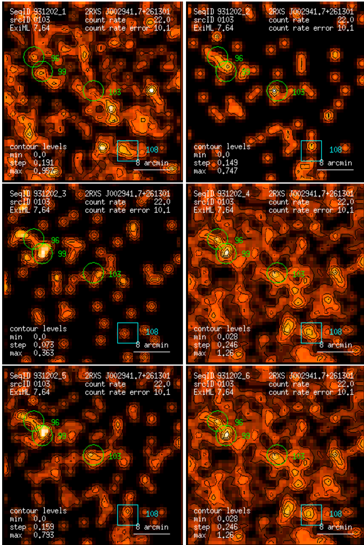
Figure 103: RASS 931202: detection 0103: band rate images, Gaussian filter: (1) PSPC channels 11 – 41, (2) 52 – 90, (3) 91 – 201, (4) 11 – 235, (5) 52 – 201, (6) 11 – 201. Broad band rates in counts/ks. Band rate contour levels in counts/ks/arcmin 2 .
