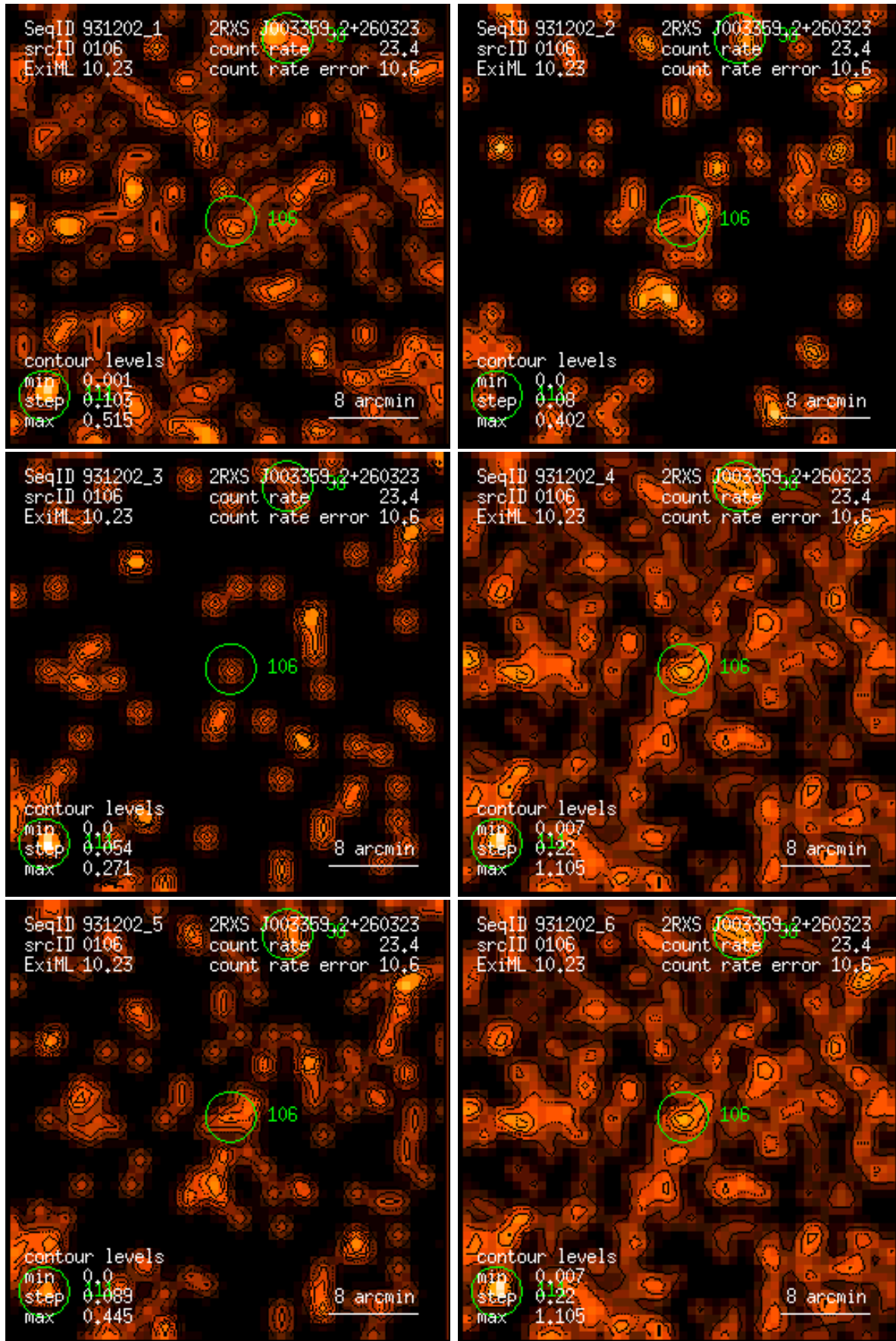
Figure 106: RASS 931202: detection 0106: band rate images, Gaussian filter: (1) PSPC channels 11 – 41, (2) 52 – 90, (3) 91 – 201, (4) 11 – 235, (5) 52 – 201, (6) 11 – 201. Broad band rates in counts/ks. Band rate contour levels in counts/ks/arcmin 2 .
