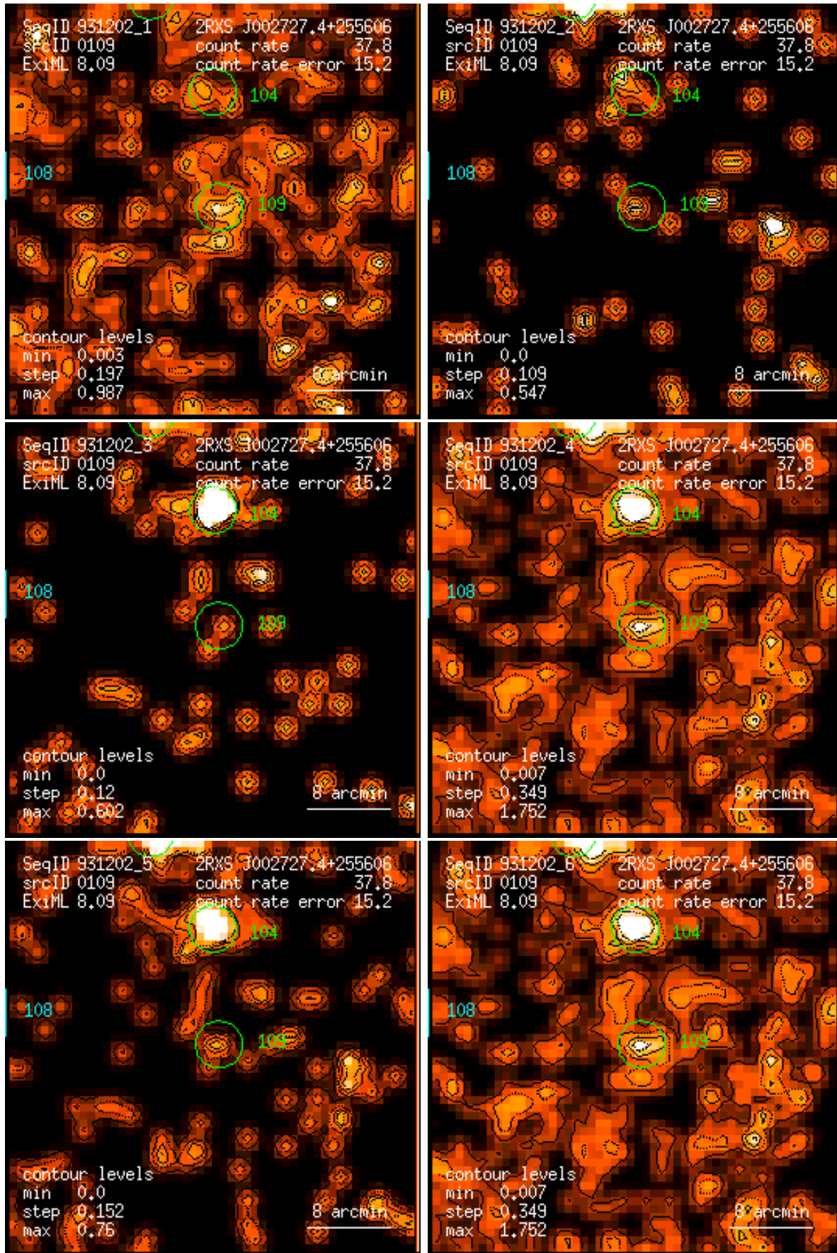
Figure 109: RASS 931202: detection 0109: band rate images, Gaussian filter: (1) PSPC channels 11 – 41, (2) 52 – 90, (3) 91 – 201, (4) 11 – 235, (5) 52 – 201, (6) 11 – 201. Broad band rates in counts/ks. Band rate contour levels in counts/ks/arcmin 2 .
