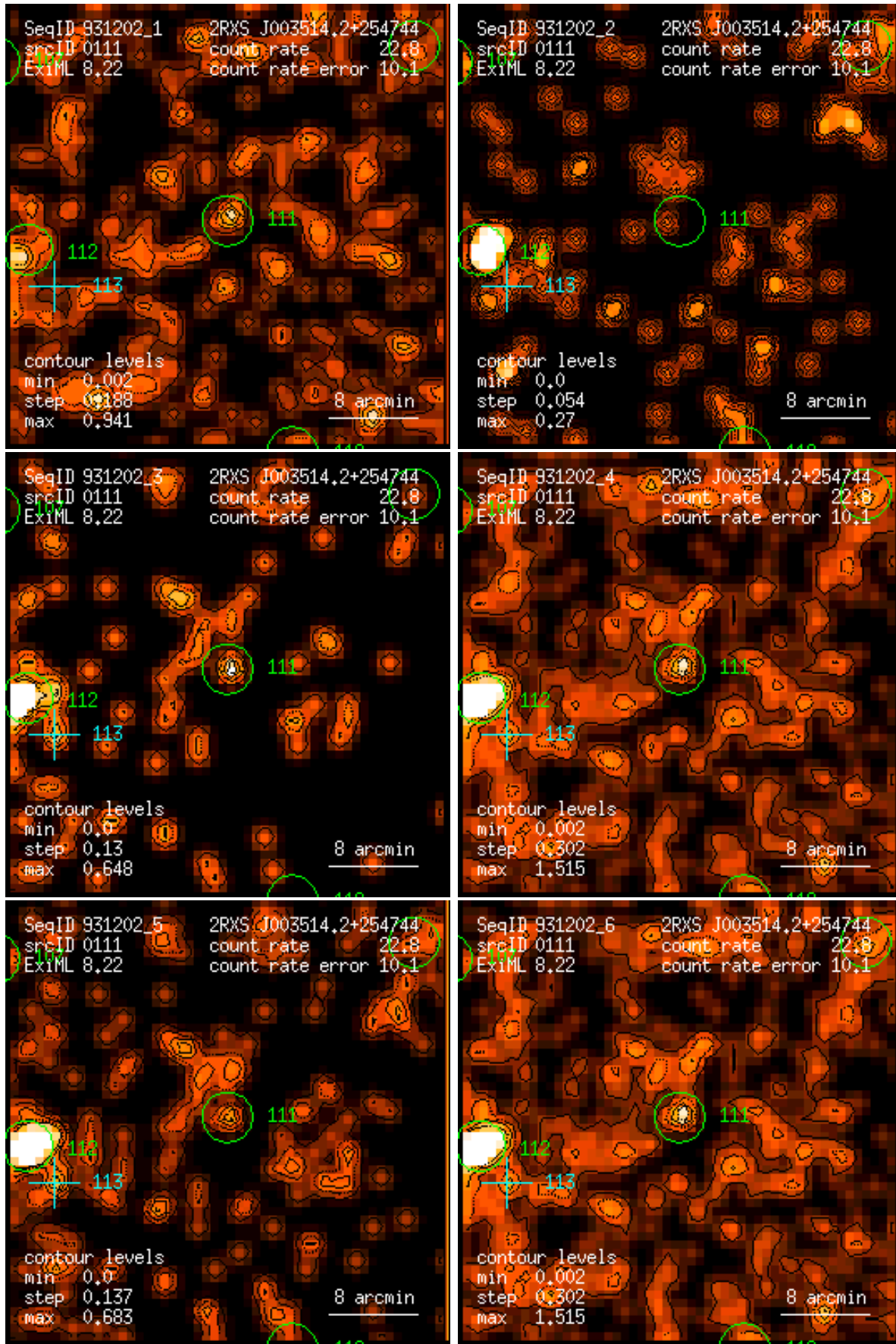
Figure 111: RASS 931202: detection 0111: band rate images, Gaussian filter: (1) PSPC channels 11 – 41, (2) 52 – 90, (3) 91 – 201, (4) 11 – 235, (5) 52 – 201, (6) 11 – 201. Broad band rates in counts/ks. Band rate contour levels in counts/ks/arcmin 2 .
