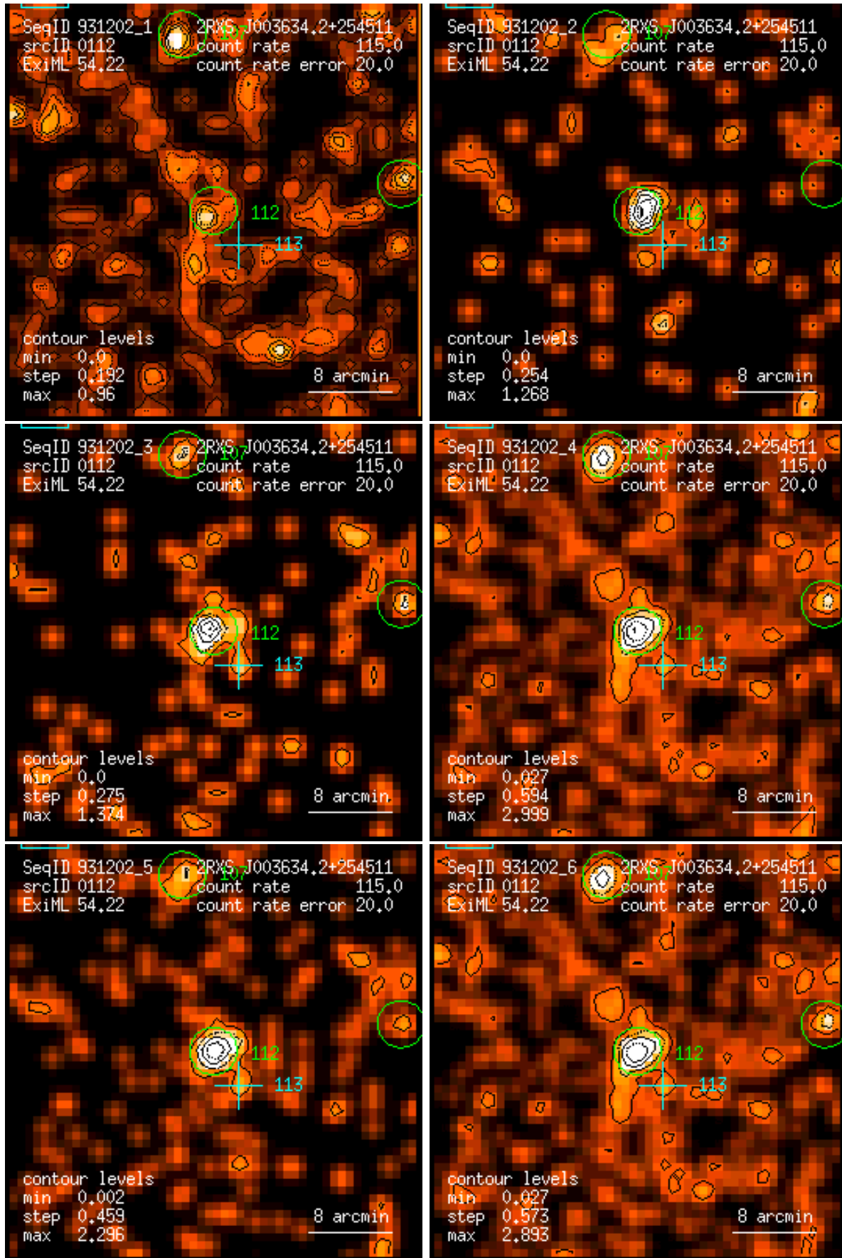
Figure 112: RASS 931202: detection 0112: band rate images, Gaussian filter: (1) PSPC channels 11 – 41, (2) 52 – 90, (3) 91 – 201, (4) 11 – 235, (5) 52 – 201, (6) 11 – 201. Broad band rates in counts/ks. Band rate contour levels in counts/ks/arcmin 2 .
