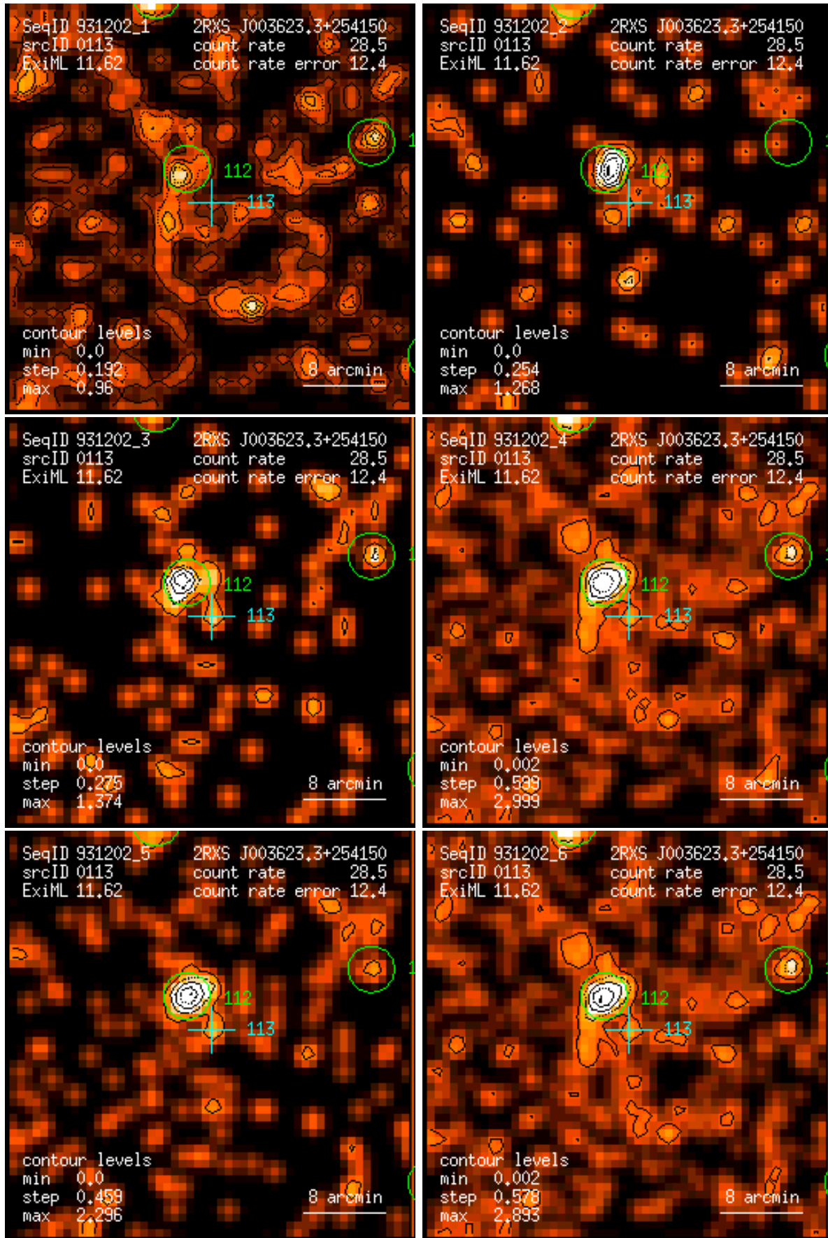
Figure 113: RASS 931202: detection 0113: band rate images, Gaussian filter: (1) PSPC channels 11 – 41, (2) 52 – 90, (3) 91 – 201, (4) 11 – 235, (5) 52 – 201, (6) 11 – 201. Broad band rates in counts/ks. Band rate contour levels in counts/ks/arcmin 2 .
