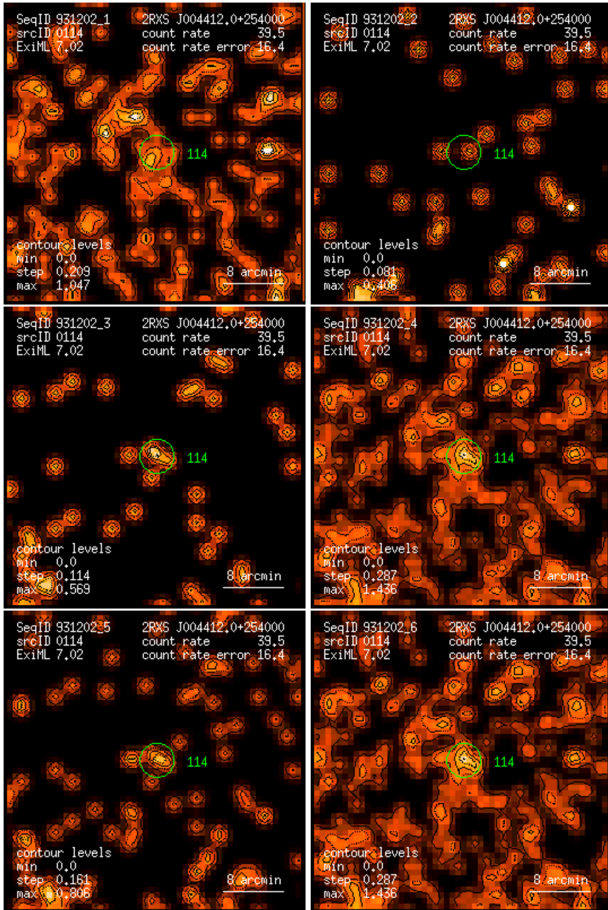
Figure 114: RASS 931202: detection 0114: band rate images, Gaussian filter: (1) PSPC channels 11 – 41, (2) 52 – 90, (3) 91 – 201, (4) 11 – 235, (5) 52 – 201, (6) 11 – 201. Broad band rates in counts/ks. Band rate contour levels in counts/ks/arcmin 2 .
