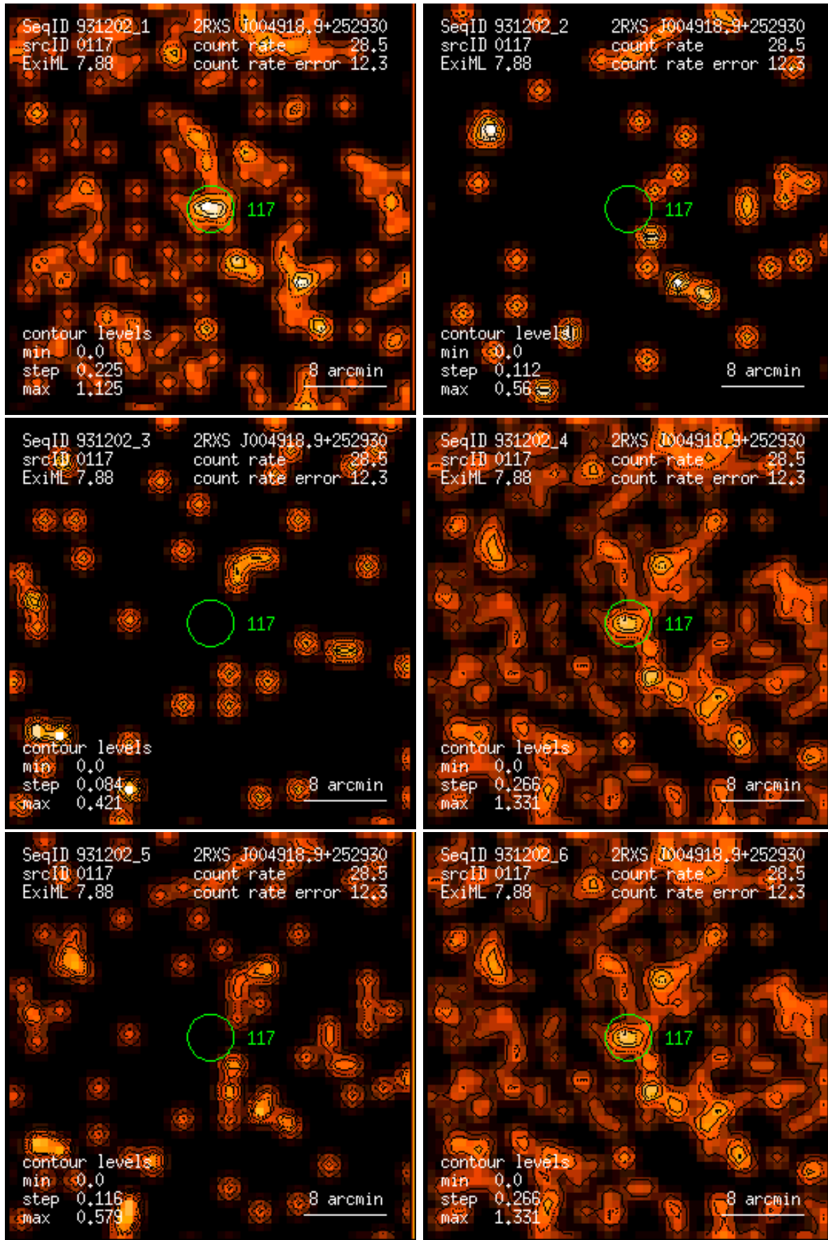
Figure 117: RASS 931202: detection 0117: band rate images, Gaussian filter: (1) PSPC channels 11 – 41, (2) 52 – 90, (3) 91 – 201, (4) 11 – 235, (5) 52 – 201, (6) 11 – 201. Broad band rates in counts/ks. Band rate contour levels in counts/ks/arcmin 2 .
