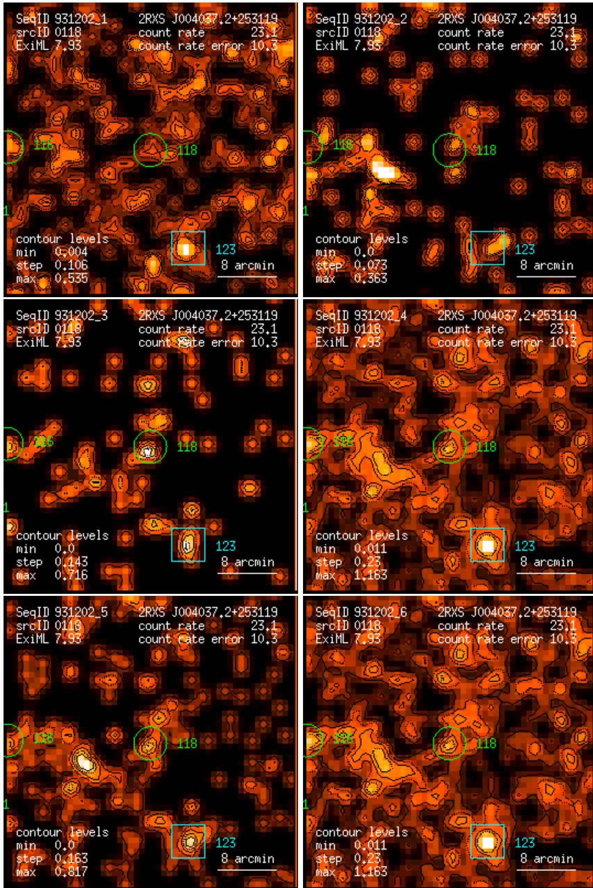
Figure 118: RASS 931202: detection 0118: band rate images, Gaussian filter: (1) PSPC channels 11 – 41, (2) 52 – 90, (3) 91 – 201, (4) 11 – 235, (5) 52 – 201, (6) 11 – 201. Broad band rates in counts/ks. Band rate contour levels in counts/ks/arcmin 2 .
