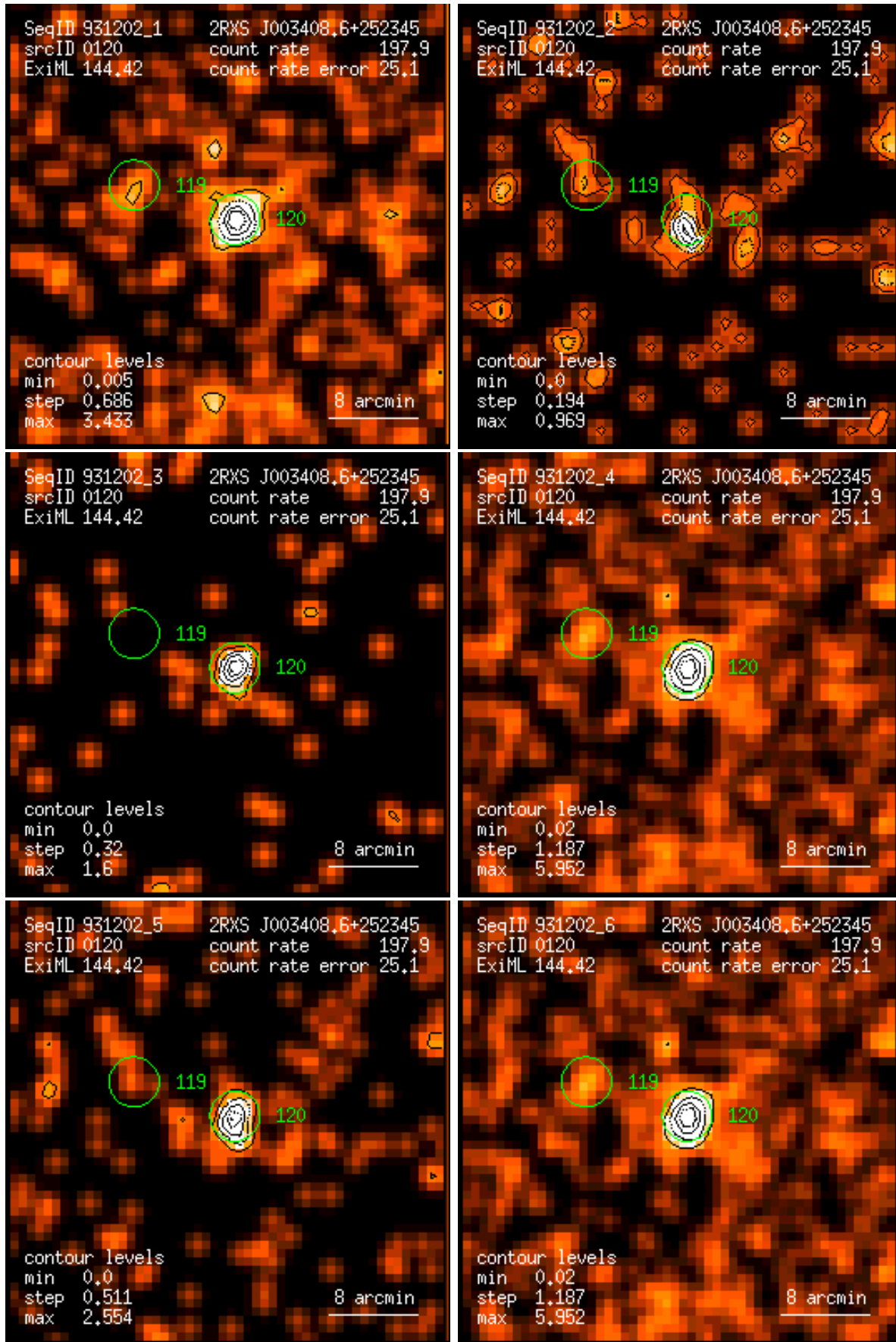
Figure 120: RASS 931202: detection 0120: band rate images, Gaussian filter: (1) PSPC channels 11 – 41, (2) 52 – 90, (3) 91 – 201, (4) 11 – 235, (5) 52 – 201, (6) 11 – 201. Broad band rates in counts/ks. Band rate contour levels in counts/ks/arcmin 2 .
