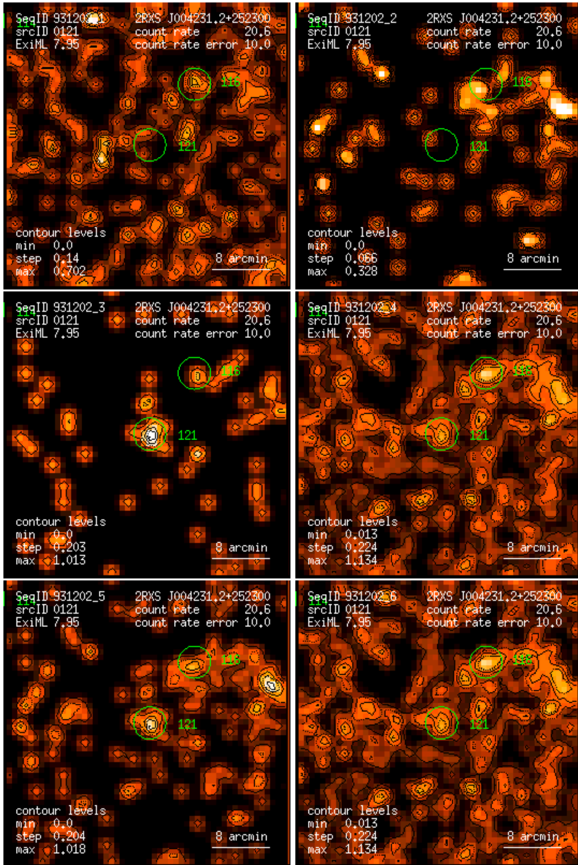
Figure 121: RASS 931202: detection 0121: band rate images, Gaussian filter: (1) PSPC channels 11 – 41, (2) 52 – 90, (3) 91 – 201, (4) 11 – 235, (5) 52 – 201, (6) 11 – 201. Broad band rates in counts/ks. Band rate contour levels in counts/ks/arcmin 2 .
