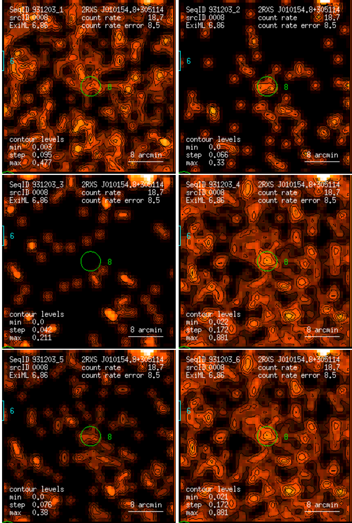
Figure 8: RASS 931203: detection 0008: band rate images, Gaussian filter: (1) PSPC channels 11 – 41, (2) 52 – 90, (3) 91 – 201, (4) 11 – 235, (5) 52 – 201, (6) 11 – 201. Broad band rates in counts/ks. Band rate contour levels in counts/ks/arcmin 2 .
