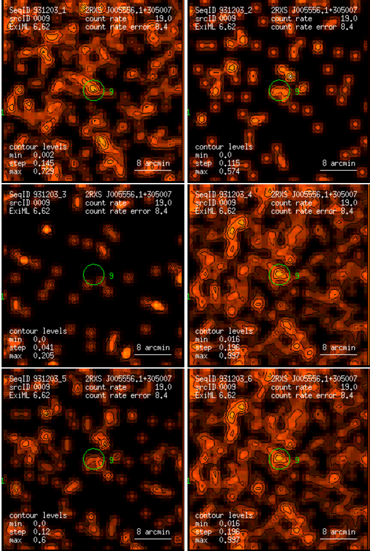
Figure 9: RASS 931203: detection 0009: band rate images, Gaussian filter: (1) PSPC channels 11 – 41, (2) 52 – 90, (3) 91 – 201, (4) 11 – 235, (5) 52 – 201, (6) 11 – 201. Broad band rates in counts/ks. Band rate contour levels in counts/ks/arcmin 2 .
