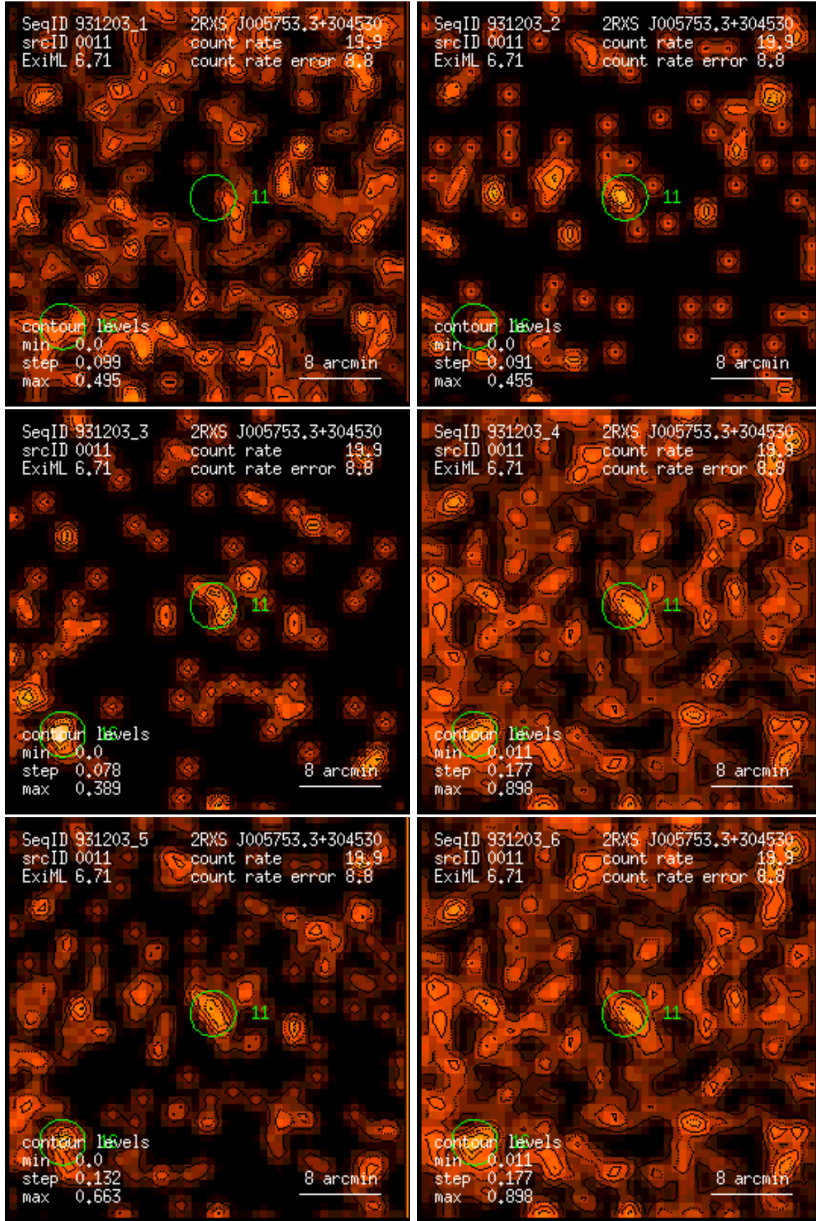
Figure 11: RASS 931203: detection 0011: band rate images, Gaussian filter: (1) PSPC channels 11 – 41, (2) 52 – 90, (3) 91 – 201, (4) 11 – 235, (5) 52 – 201, (6) 11 – 201. Broad band rates in counts/ks. Band rate contour levels in counts/ks/arcmin 2 .
