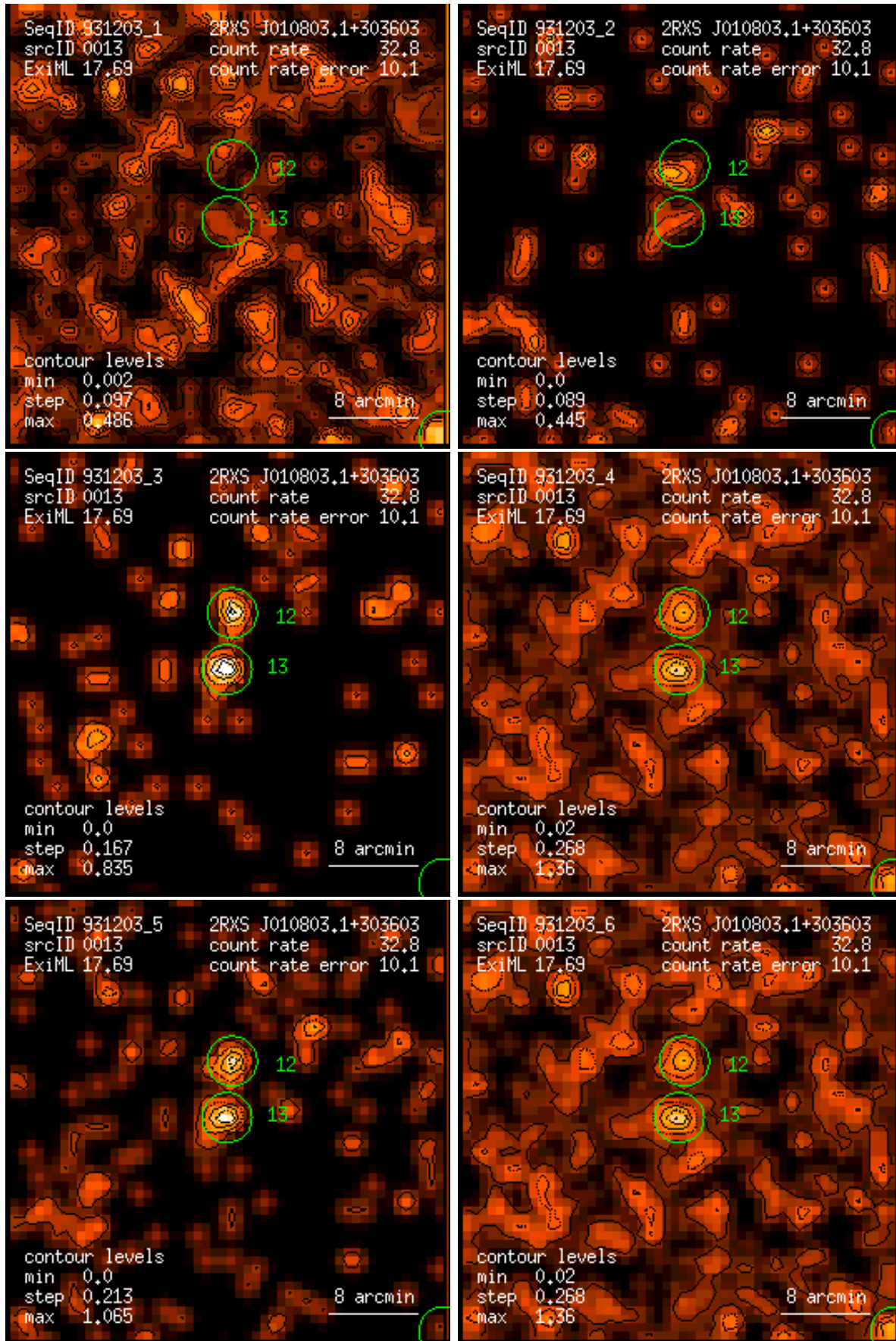
Figure 13: RASS 931203: detection 0013: band rate images, Gaussian filter: (1) PSPC channels 11 – 41, (2) 52 – 90, (3) 91 – 201, (4) 11 – 235, (5) 52 – 201, (6) 11 – 201. Broad band rates in counts/ks. Band rate contour levels in counts/ks/arcmin 2 .
