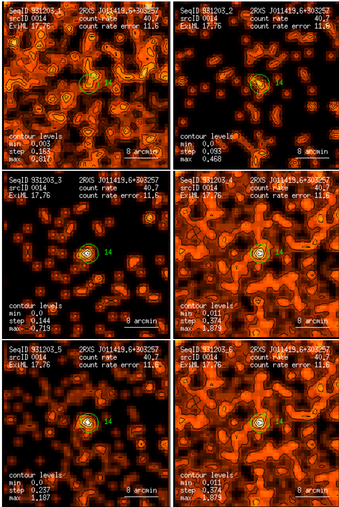
Figure 14: RASS 931203: detection 0014: band rate images, Gaussian filter: (1) PSPC channels 11 – 41, (2) 52 – 90, (3) 91 – 201, (4) 11 – 235, (5) 52 – 201, (6) 11 – 201. Broad band rates in counts/ks. Band rate contour levels in counts/ks/arcmin 2 .
