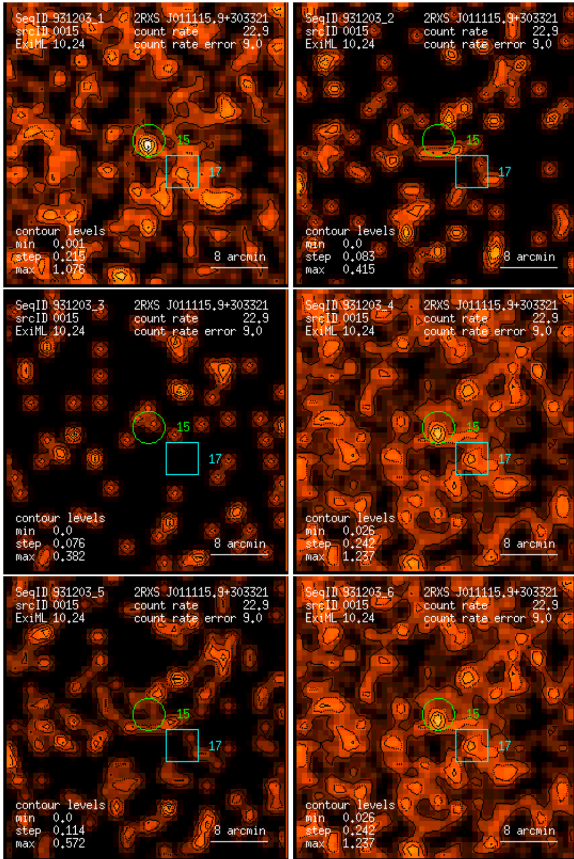
Figure 15: RASS 931203: detection 0015: band rate images, Gaussian filter: (1) PSPC channels 11 – 41, (2) 52 – 90, (3) 91 – 201, (4) 11 – 235, (5) 52 – 201, (6) 11 – 201. Broad band rates in counts/ks. Band rate contour levels in counts/ks/arcmin 2 .
