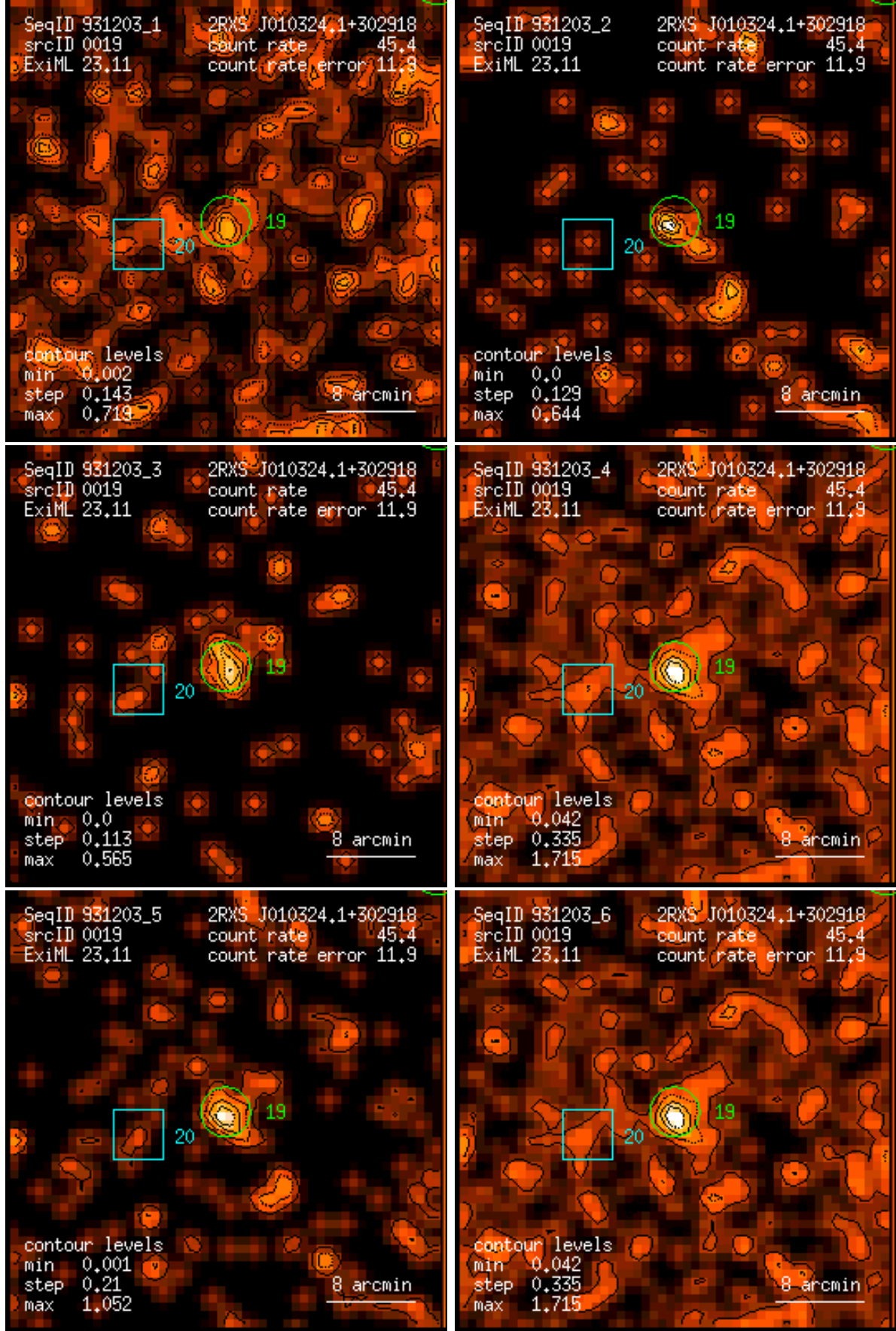
Figure 19: RASS 931203: detection 0019: band rate images, Gaussian filter: (1) PSPC channels 11 – 41, (2) 52 – 90, (3) 91 – 201, (4) 11 – 235, (5) 52 – 201, (6) 11 – 201. Broad band rates in counts/ks. Band rate contour levels in counts/ks/arcmin 2 .
