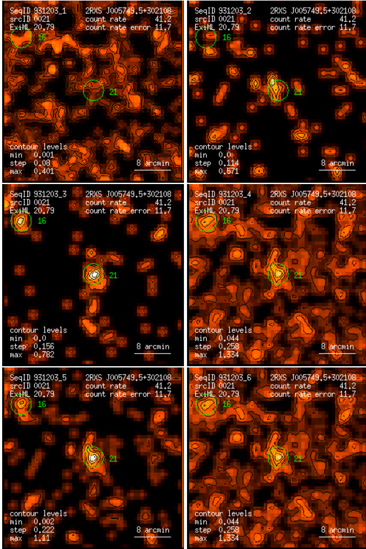
Figure 21: RASS 931203: detection 0021: band rate images, Gaussian filter: (1) PSPC channels 11 – 41, (2) 52 – 90, (3) 91 – 201, (4) 11 – 235, (5) 52 – 201, (6) 11 – 201. Broad band rates in counts/ks. Band rate contour levels in counts/ks/arcmin 2 .
