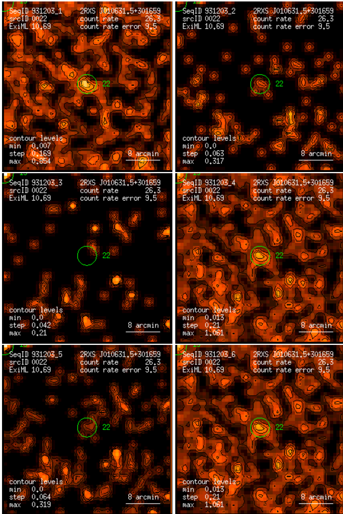
Figure 22: RASS 931203: detection 0022: band rate images, Gaussian filter: (1) PSPC channels 11 – 41, (2) 52 – 90, (3) 91 – 201, (4) 11 – 235, (5) 52 – 201, (6) 11 – 201. Broad band rates in counts/ks. Band rate contour levels in counts/ks/arcmin 2 .
