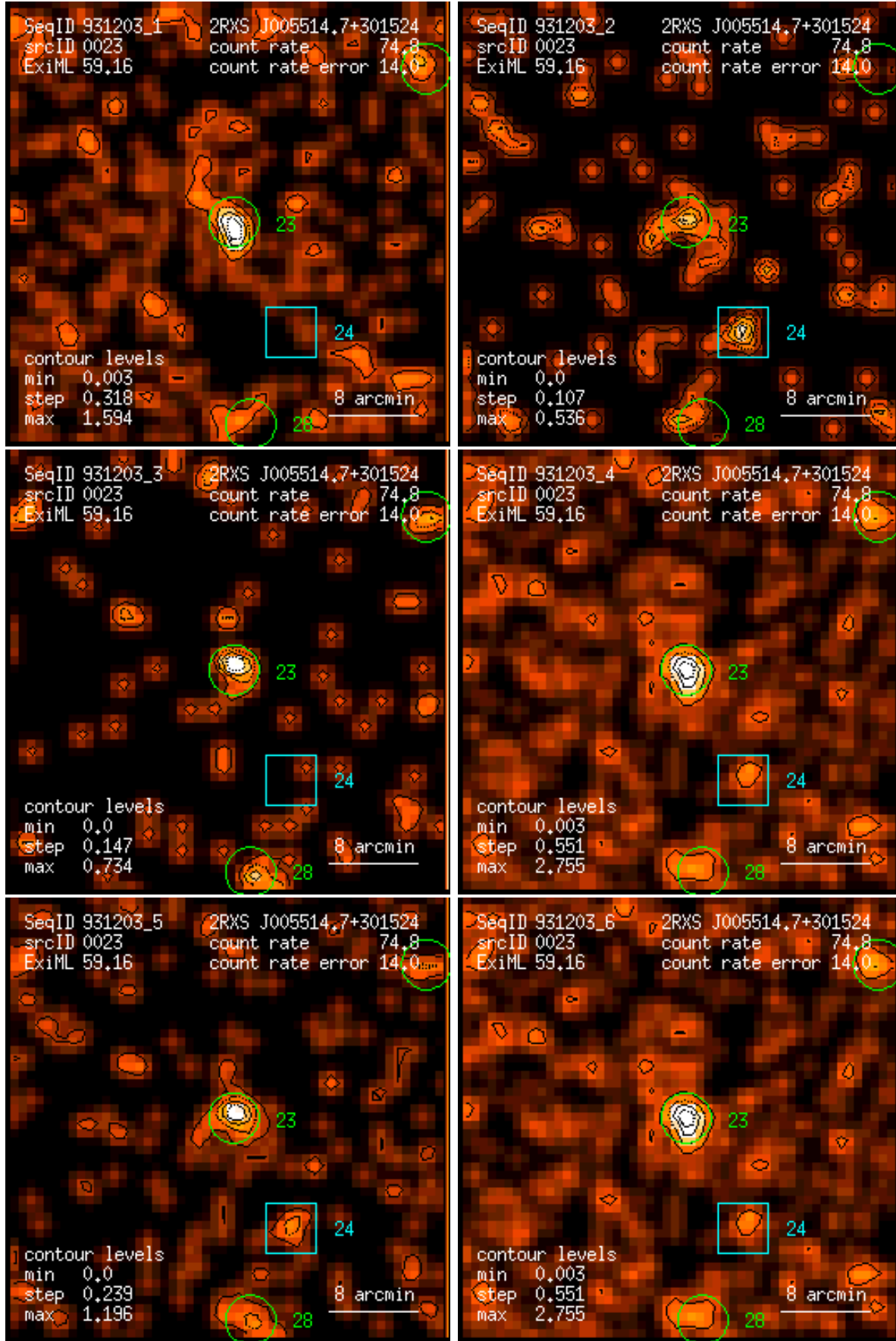
Figure 23: RASS 931203: detection 0023: band rate images, Gaussian filter: (1) PSPC channels 11 – 41, (2) 52 – 90, (3) 91 – 201, (4) 11 – 235, (5) 52 – 201, (6) 11 – 201. Broad band rates in counts/ks. Band rate contour levels in counts/ks/arcmin 2 .
