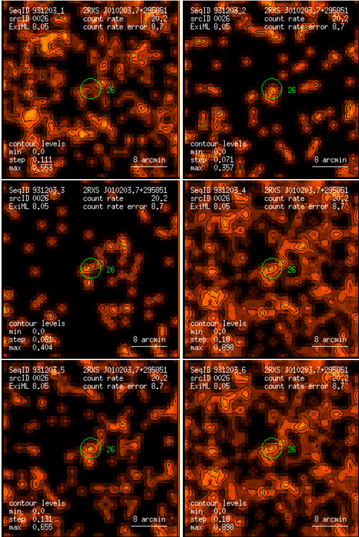
Figure 26: RASS 931203: detection 0026: band rate images, Gaussian filter: (1) PSPC channels 11 – 41, (2) 52 – 90, (3) 91 – 201, (4) 11 – 235, (5) 52 – 201, (6) 11 – 201. Broad band rates in counts/ks. Band rate contour levels in counts/ks/arcmin 2 .
