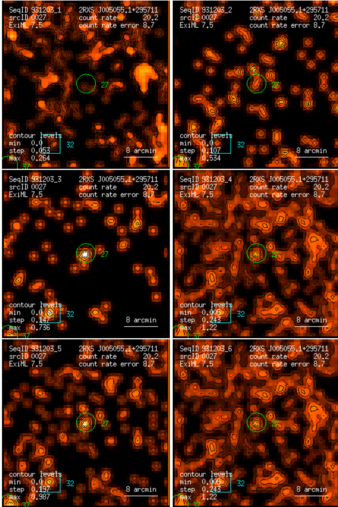
Figure 27: RASS 931203: detection 0027: band rate images, Gaussian filter: (1) PSPC channels 11 – 41, (2) 52 – 90, (3) 91 – 201, (4) 11 – 235, (5) 52 – 201, (6) 11 – 201. Broad band rates in counts/ks. Band rate contour levels in counts/ks/arcmin 2 .
