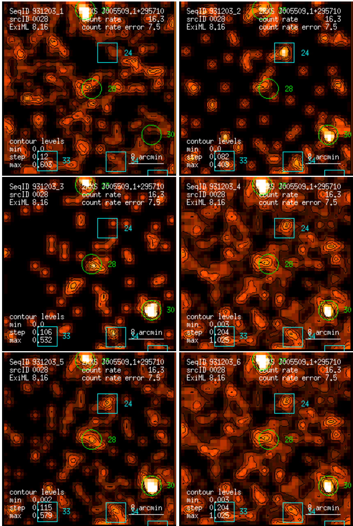
Figure 28: RASS 931203: detection 0028: band rate images, Gaussian filter: (1) PSPC channels 11 – 41, (2) 52 – 90, (3) 91 – 201, (4) 11 – 235, (5) 52 – 201, (6) 11 – 201. Broad band rates in counts/ks. Band rate contour levels in counts/ks/arcmin 2 .
