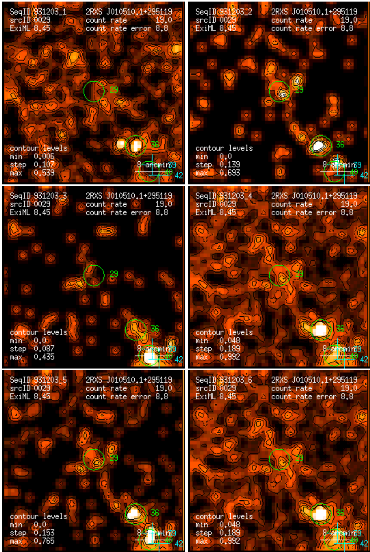
Figure 29: RASS 931203: detection 0029: band rate images, Gaussian filter: (1) PSPC channels 11 – 41, (2) 52 – 90, (3) 91 – 201, (4) 11 – 235, (5) 52 – 201, (6) 11 – 201. Broad band rates in counts/ks. Band rate contour levels in counts/ks/arcmin 2 .
