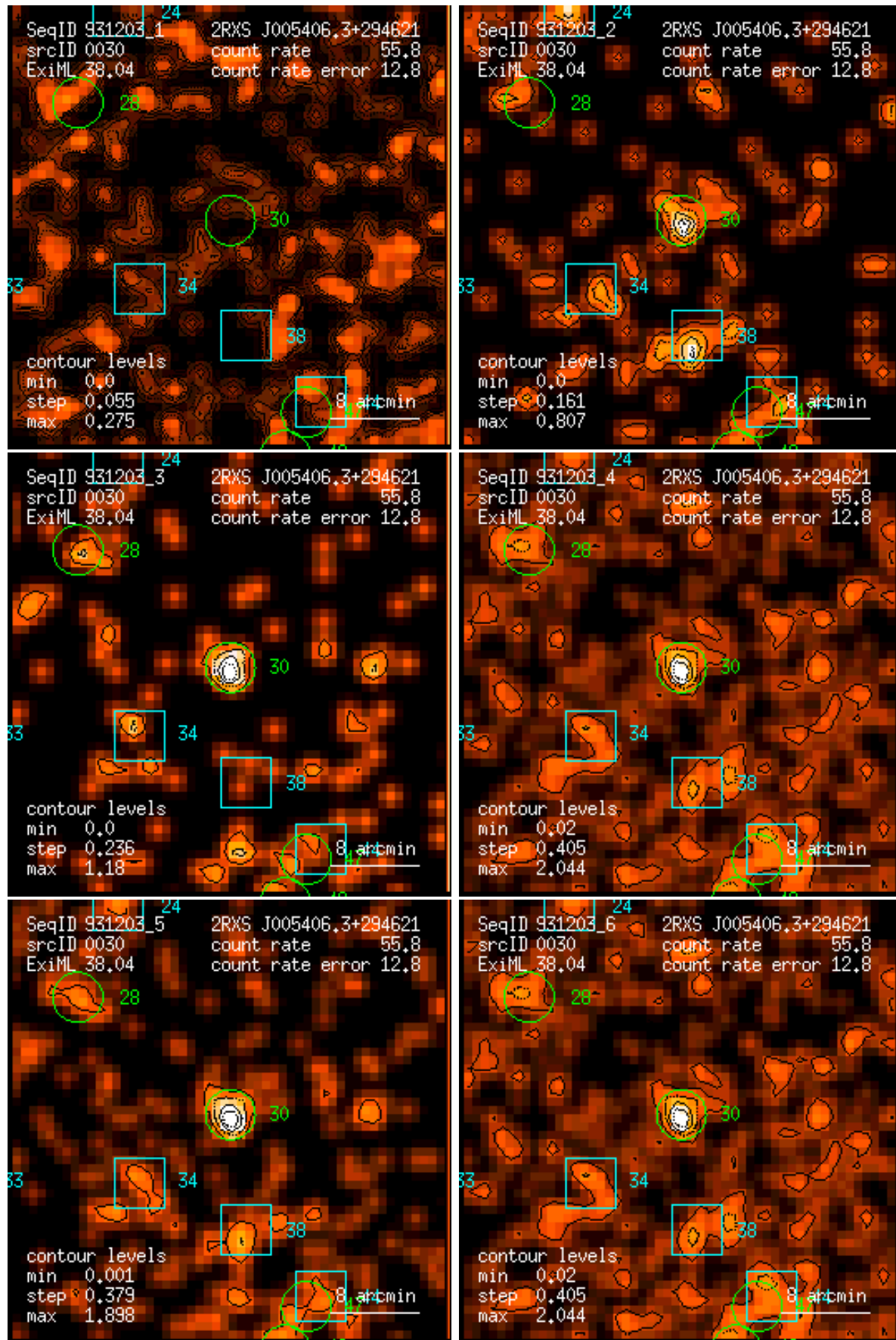
Figure 30: RASS 931203: detection 0030: band rate images, Gaussian filter: (1) PSPC channels 11 – 41, (2) 52 – 90, (3) 91 – 201, (4) 11 – 235, (5) 52 – 201, (6) 11 – 201. Broad band rates in counts/ks. Band rate contour levels in counts/ks/arcmin 2 .
