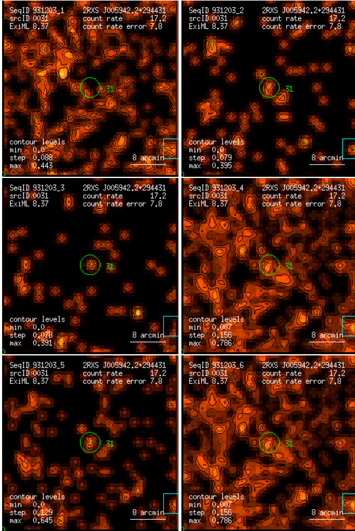
Figure 31: RASS 931203: detection 0031: band rate images, Gaussian filter: (1) PSPC channels 11 – 41, (2) 52 – 90, (3) 91 – 201, (4) 11 – 235, (5) 52 – 201, (6) 11 – 201. Broad band rates in counts/ks. Band rate contour levels in counts/ks/arcmin 2 .
