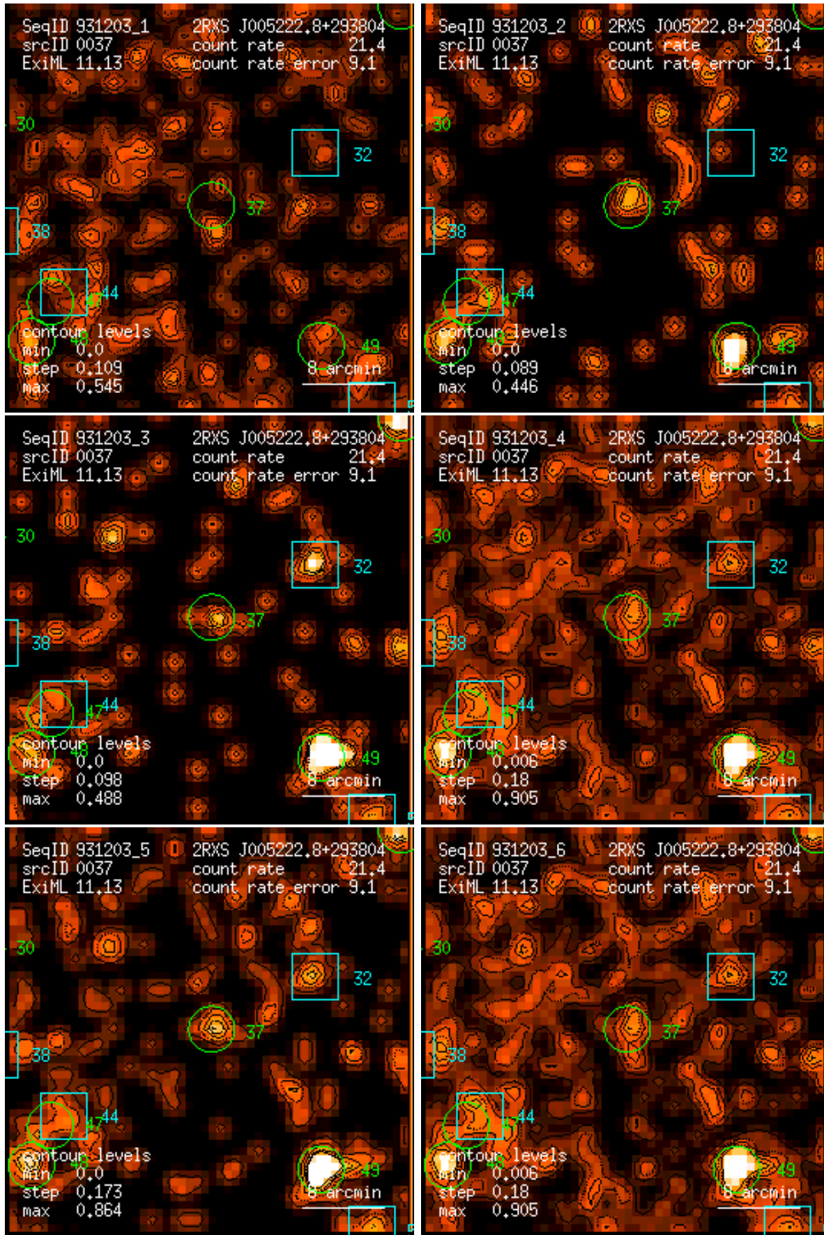
Figure 37: RASS 931203: detection 0037: band rate images, Gaussian filter: (1) PSPC channels 11 – 41, (2) 52 – 90, (3) 91 – 201, (4) 11 – 235, (5) 52 – 201, (6) 11 – 201. Broad band rates in counts/ks. Band rate contour levels in counts/ks/arcmin 2 .
