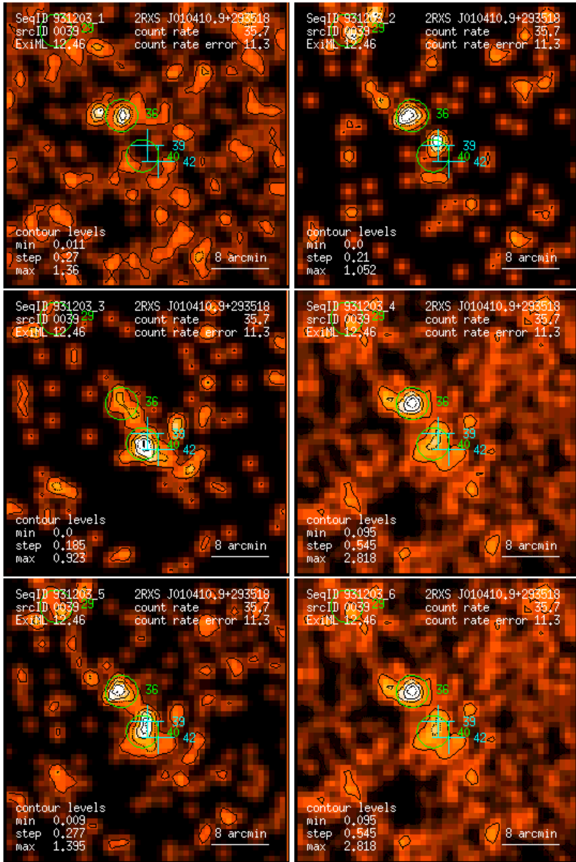
Figure 39: RASS 931203: detection 0039: band rate images, Gaussian filter: (1) PSPC channels 11 – 41, (2) 52 – 90, (3) 91 – 201, (4) 11 – 235, (5) 52 – 201, (6) 11 – 201. Broad band rates in counts/ks. Band rate contour levels in counts/ks/arcmin 2 .
