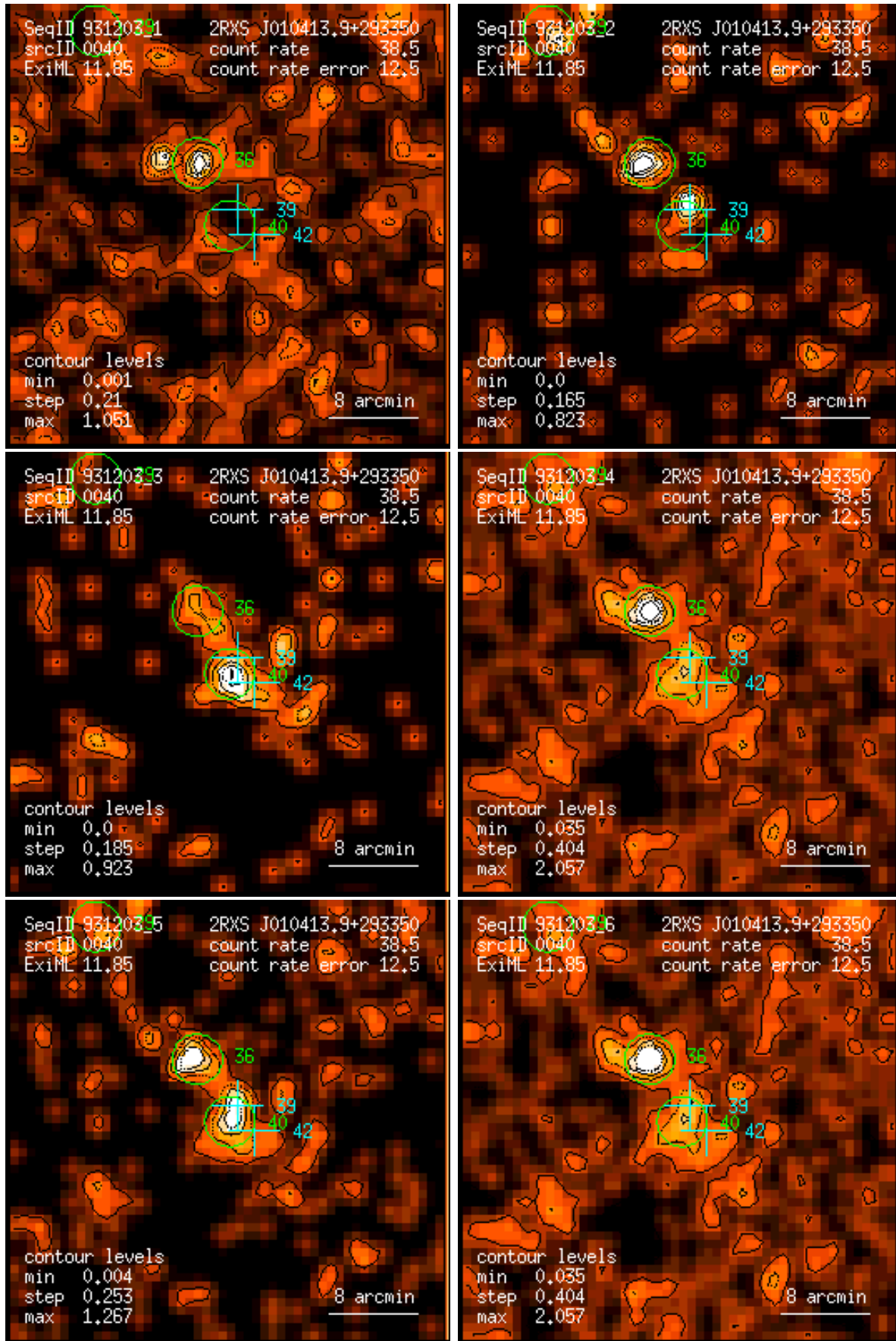
Figure 40: RASS 931203: detection 0040: band rate images, Gaussian filter: (1) PSPC channels 11 – 41, (2) 52 – 90, (3) 91 – 201, (4) 11 – 235, (5) 52 – 201, (6) 11 – 201. Broad band rates in counts/ks. Band rate contour levels in counts/ks/arcmin 2 .
