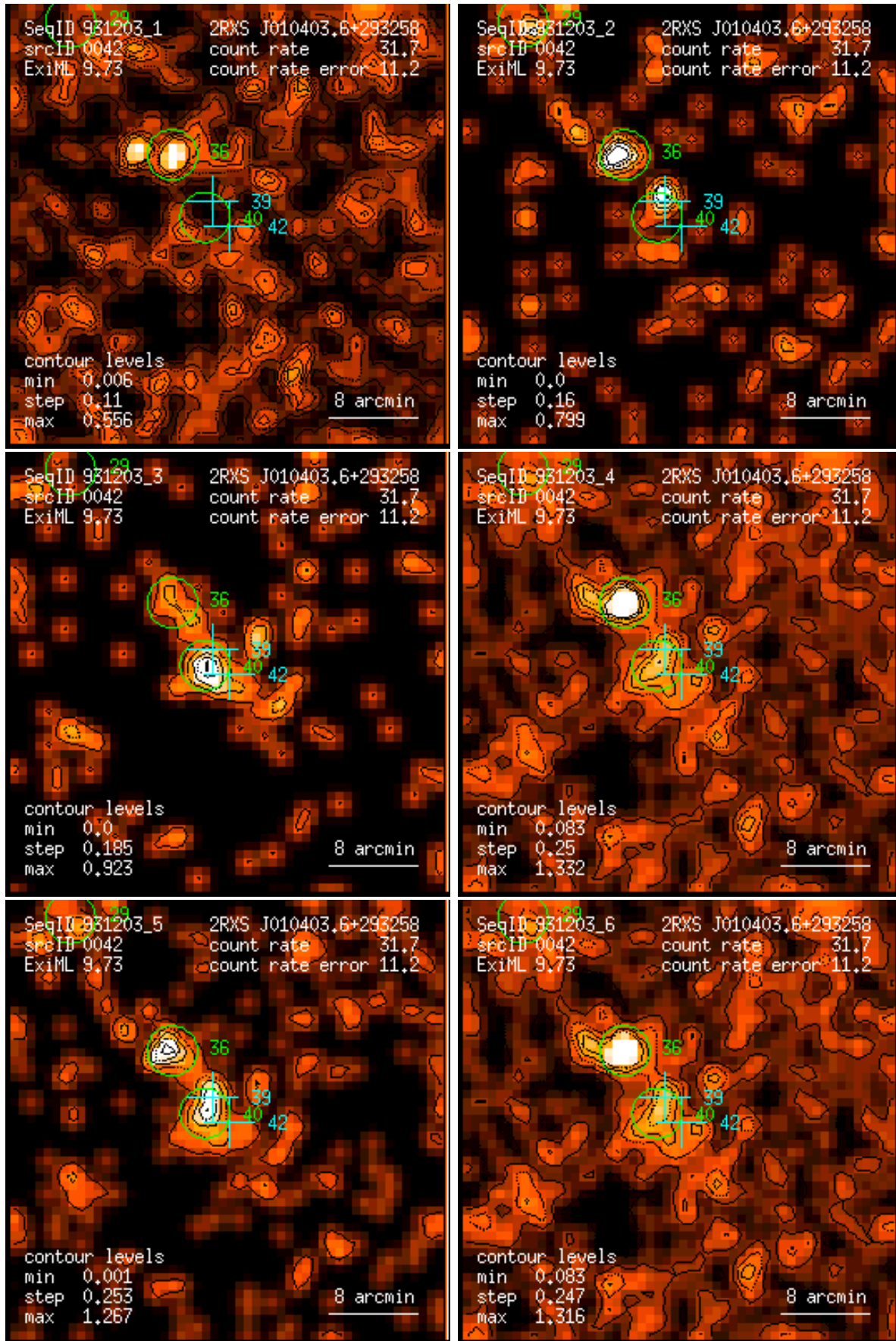
Figure 42: RASS 931203: detection 0042: band rate images, Gaussian filter: (1) PSPC channels 11 – 41, (2) 52 – 90, (3) 91 – 201, (4) 11 – 235, (5) 52 – 201, (6) 11 – 201. Broad band rates in counts/ks. Band rate contour levels in counts/ks/arcmin 2 .
