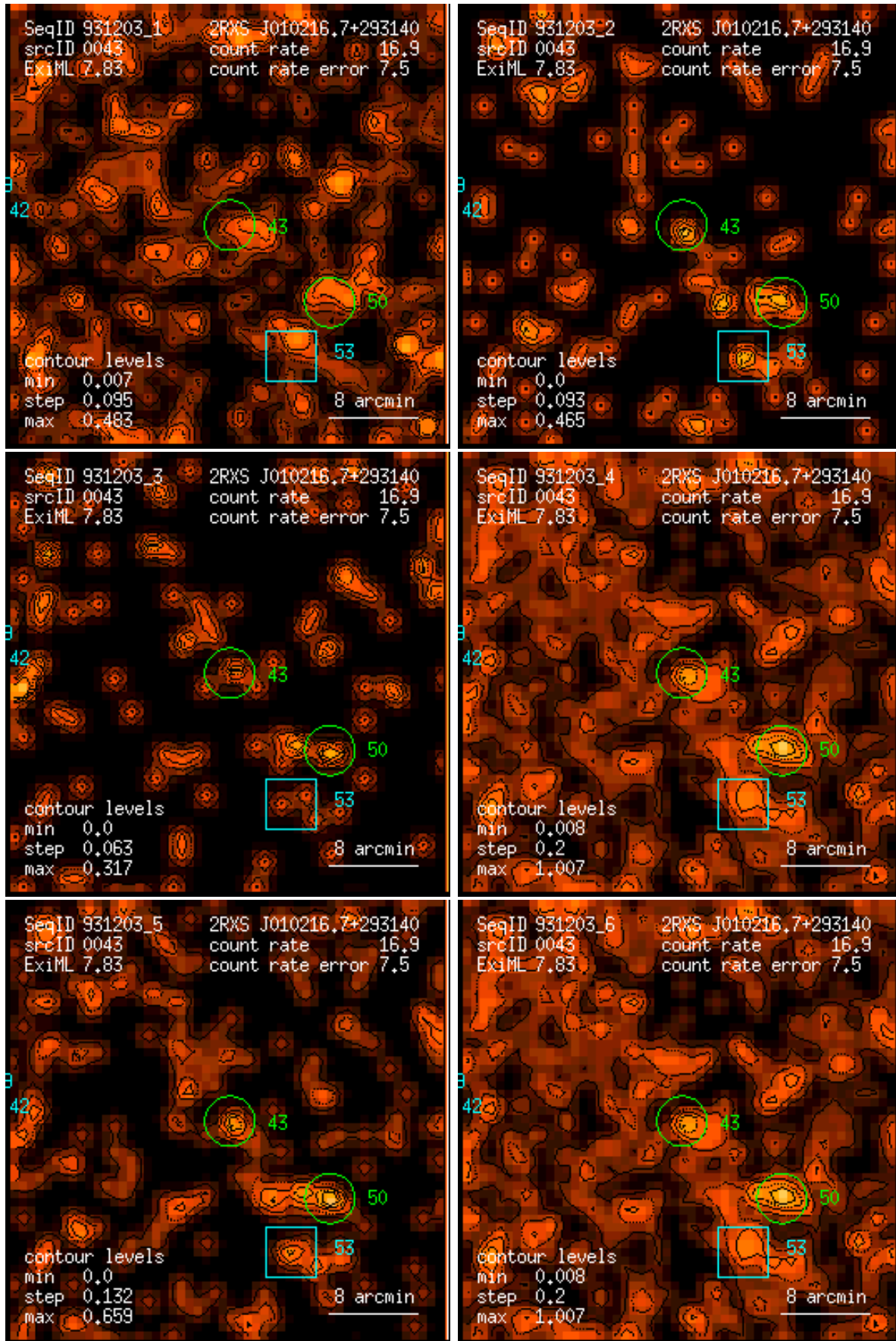
Figure 43: RASS 931203: detection 0043: band rate images, Gaussian filter: (1) PSPC channels 11 – 41, (2) 52 – 90, (3) 91 – 201, (4) 11 – 235, (5) 52 – 201, (6) 11 – 201. Broad band rates in counts/ks. Band rate contour levels in counts/ks/arcmin 2 .
