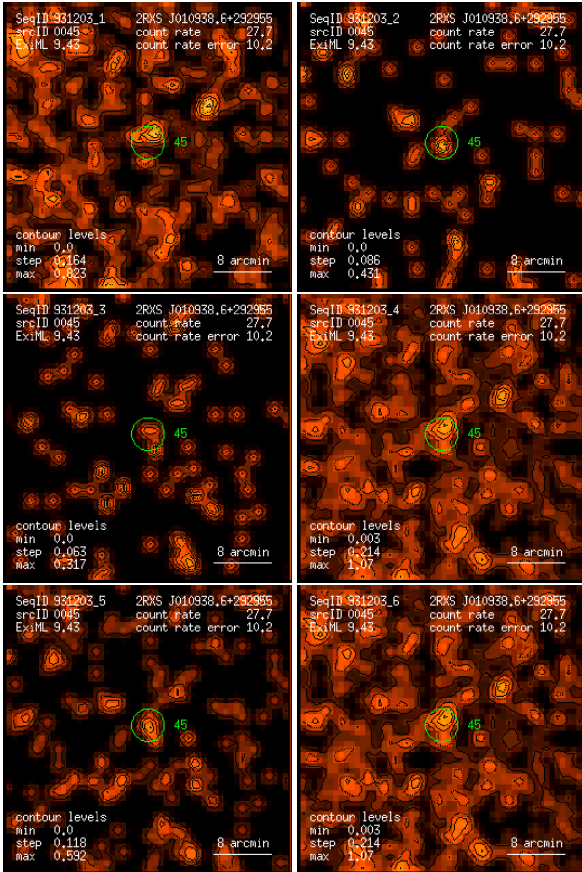
Figure 45: RASS 931203: detection 0045: band rate images, Gaussian filter: (1) PSPC channels 11 – 41, (2) 52 – 90, (3) 91 – 201, (4) 11 – 235, (5) 52 – 201, (6) 11 – 201. Broad band rates in counts/ks. Band rate contour levels in counts/ks/arcmin 2 .
