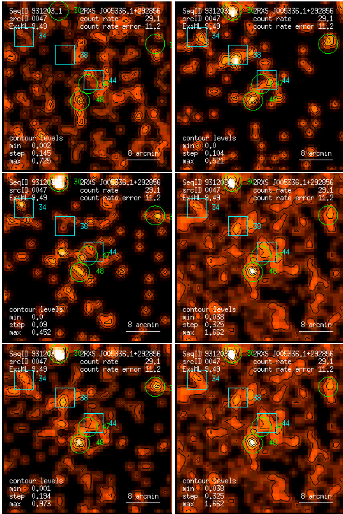
Figure 47: RASS 931203: detection 0047: band rate images, Gaussian filter: (1) PSPC channels 11 – 41, (2) 52 – 90, (3) 91 – 201, (4) 11 – 235, (5) 52 – 201, (6) 11 – 201. Broad band rates in counts/ks. Band rate contour levels in counts/ks/arcmin 2 .
