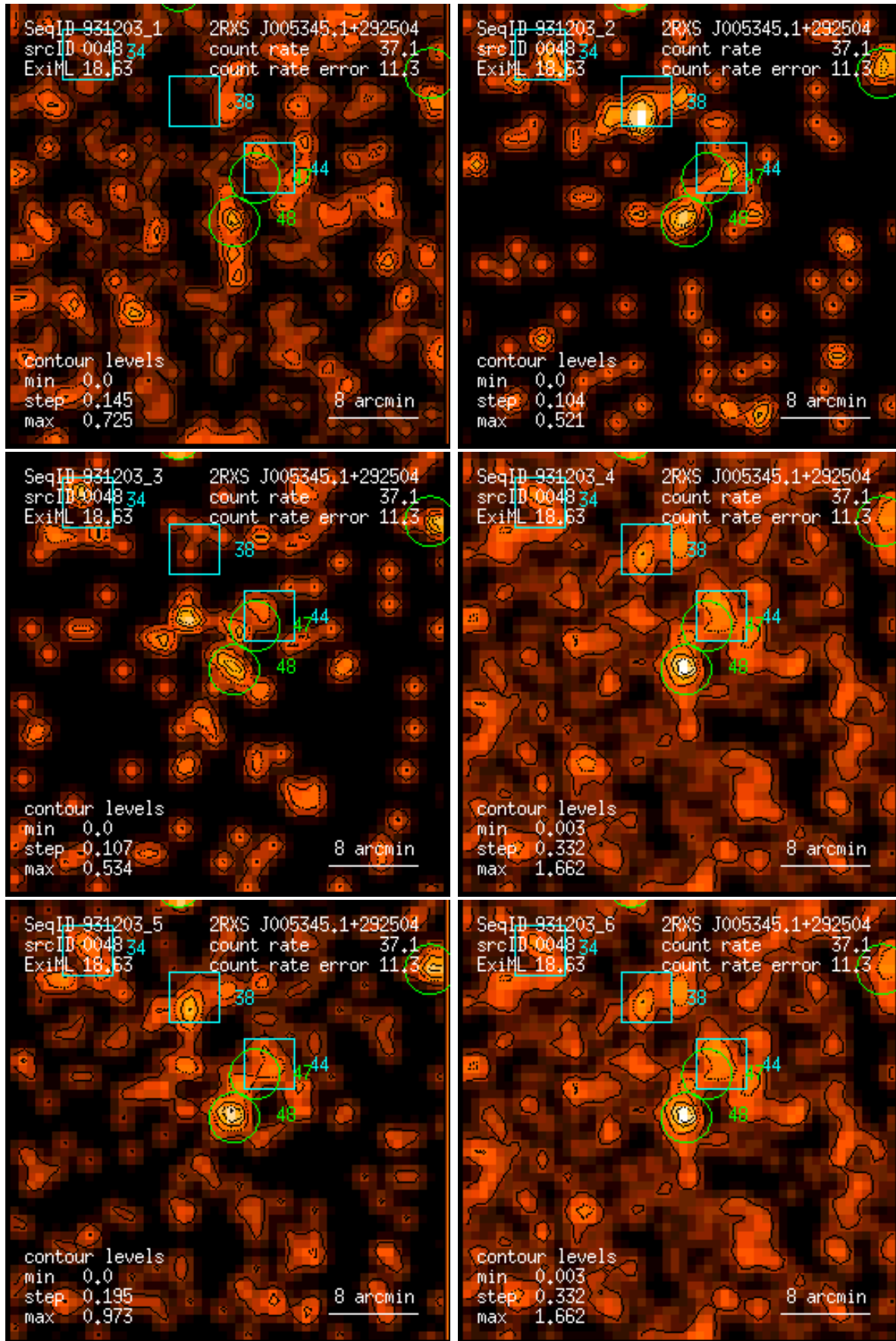
Figure 48: RASS 931203: detection 0048: band rate images, Gaussian filter: (1) PSPC channels 11 – 41, (2) 52 – 90, (3) 91 – 201, (4) 11 – 235, (5) 52 – 201, (6) 11 – 201. Broad band rates in counts/ks. Band rate contour levels in counts/ks/arcmin 2 .
